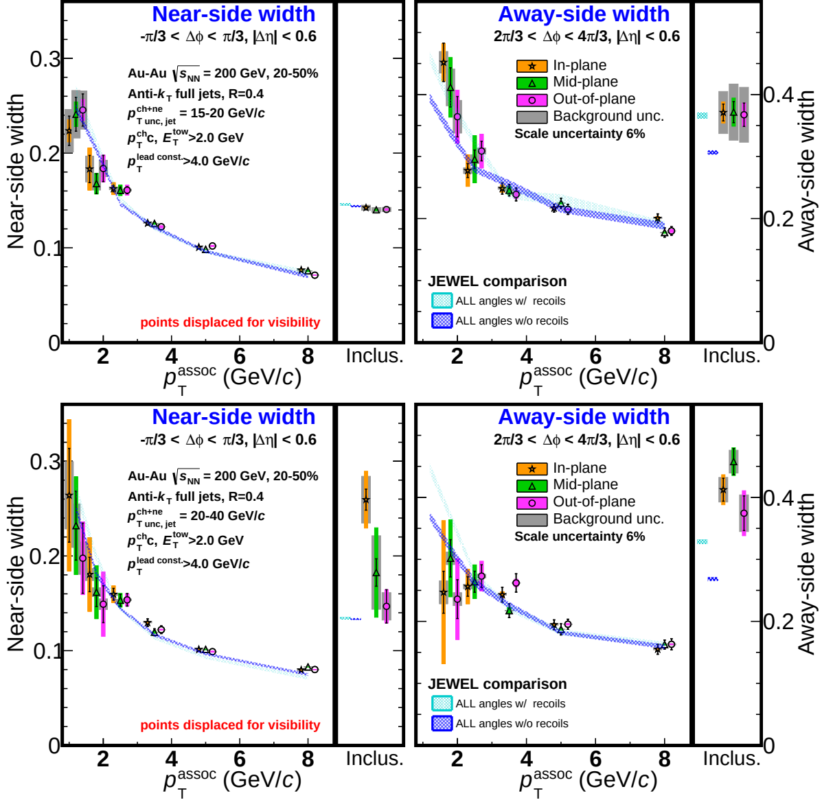
Figure 6.6: Near-side (left) and away-side (right) jet width vs p_{T,assoc} for 15-20 (top) and 20-40 GeV/c (bottom) full jets of 20-50% centrality in Au+Au collisions. The widths are extracted from the gaussian fit to the jet peak. The grey bands describe the systematic uncertainties of the background fits which are non-trivially correlated point-to-point. The colored bands are scale uncertainties from the mixed-event acceptance shape and JES correction. There is an additional 6% global scale uncertainty. Included on the far right of the near- and away-side panels is an inclusive transverse momentum bin from 1.0-10.0 GeV/c. Points are displaced for visibility.
