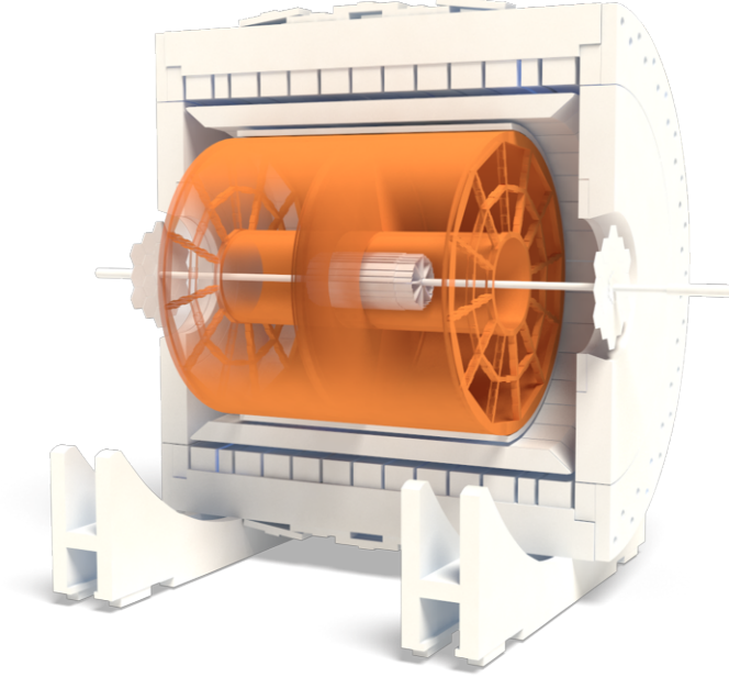
Figure 4.5: The Time Projection Chamber at STAR. Taken from [? ].
