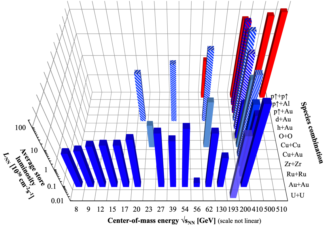
Figure 4.1: Summary of RHIC energies, species combinations, and luminosities for runs between 2000 and 2026. Taken from [? ].
