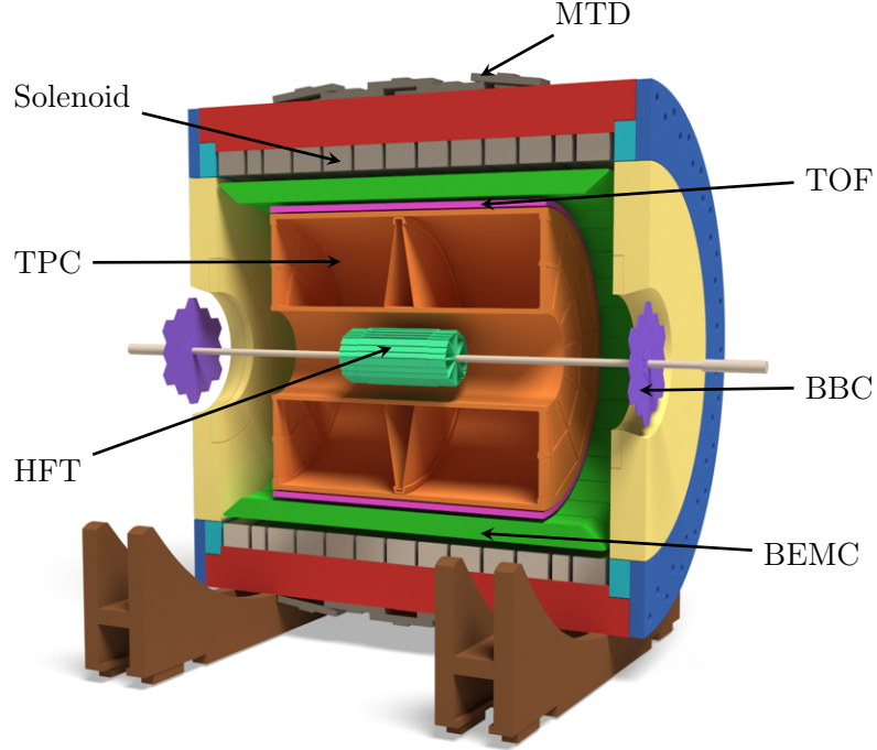
Figure 4.4: Schematic of the STAR detector, depicting the various detector subsystems.
