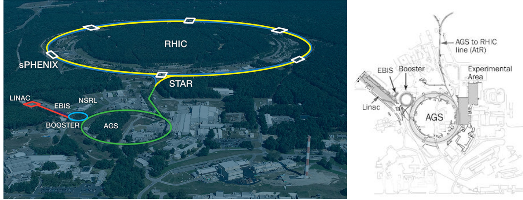
Figure 4.3: (Left) An aerial view of the Relativistic Heavy Ion Collider (RHIC), showing the locations of the facilities used for accelerating different ions, and the positions of the STAR and sPHENIX detectors. Taken from [? ].
