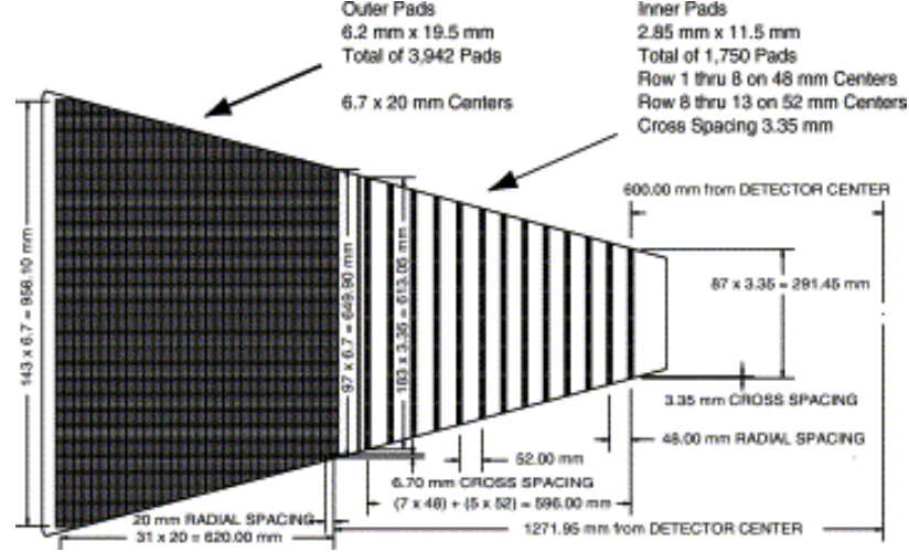
Figure 4.6: One of the twelve sectors of the TPC. Taken from [? ].
