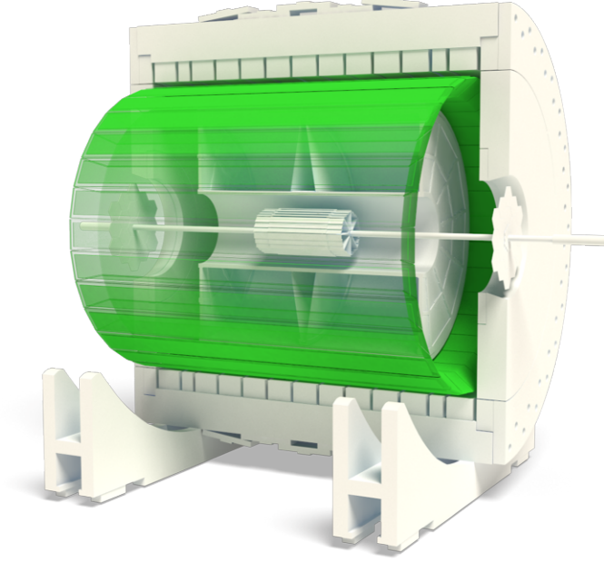
Figure 4.8: The Barrel Electromagnetic Calorimeter at STAR. Taken from [? ].
