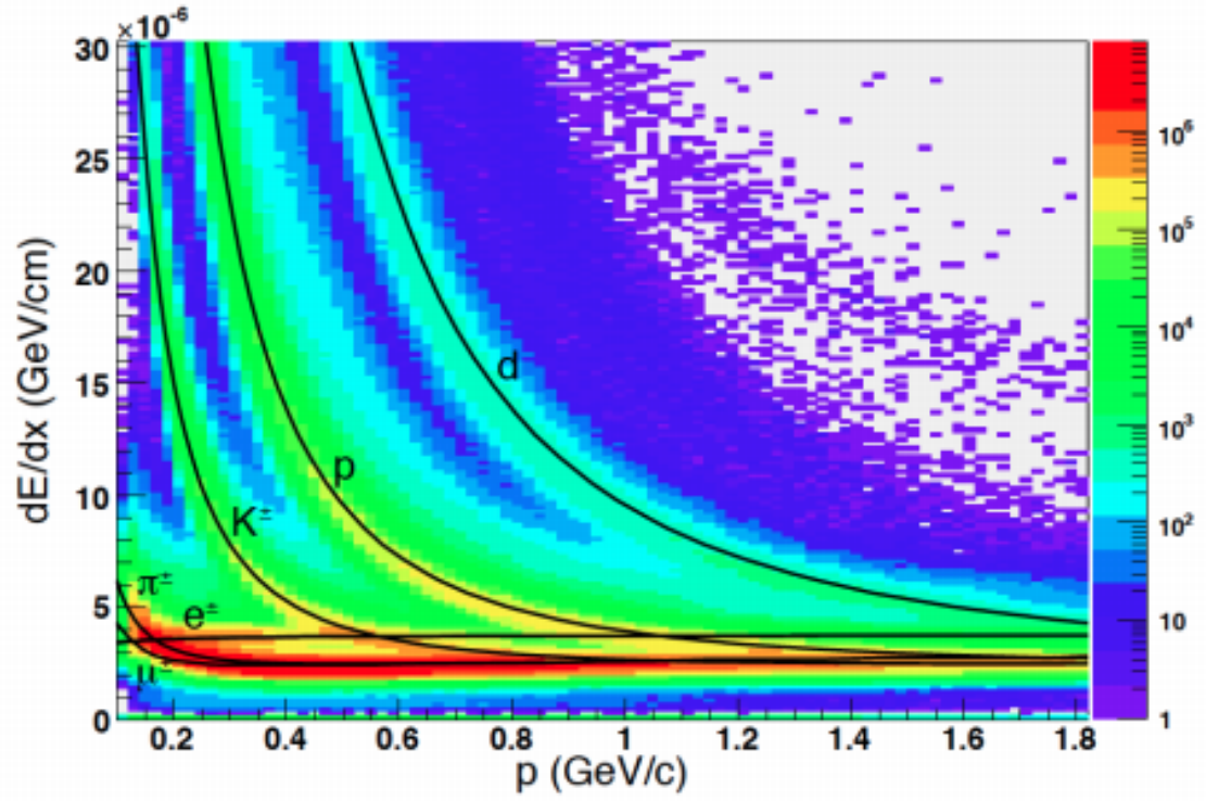
Figure 4.7: The ionisation energy loss for charged particles from TPC as a function of momenta. The letters represent different particles: \mu^\pm for muons, e^\pm for electrons, \pi^\pm for pions, K^\pm for Kaons, p for protons, and d for deuterons. The solid lines are the expected value of dE/dx for the corresponding particle species from the Bichsel function [? ].
