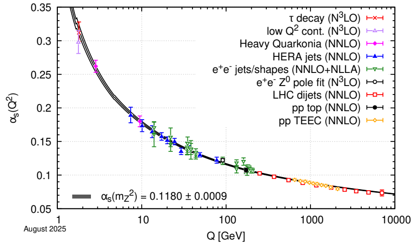
Figure 1.1: Summary of determinations of \alpha_s as a function of the energy scale Q compared to the running of the coupling computed at five loops taking as an input the current Particle Data Group (PDG) world average, \alpha_s(m_Z^2) = 0.1180 \pm 0.0009 [1]
