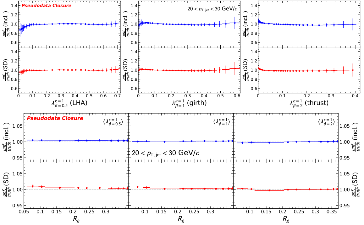
Figure 5.2: Closures for \lambda_{\beta \in \{0.5, 1, 2\}}^{\kappa=1} distributions (top) and R_g profile (bottom) shown for jets with 20 \leq p_{T,jet} < 30 \text{ GeV}/c .
