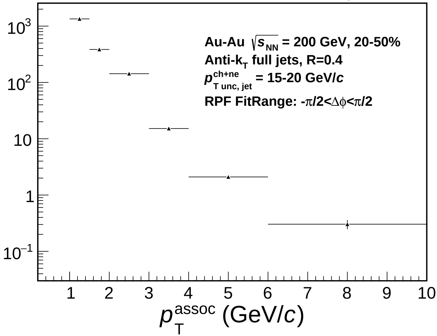
Background level vs associated hadron p_T
