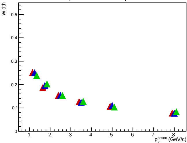
Widths vs p_T^{\text{assoc}} , Near Side, p_T^{\text{Jet, reco}} \in [15 \ 20]
