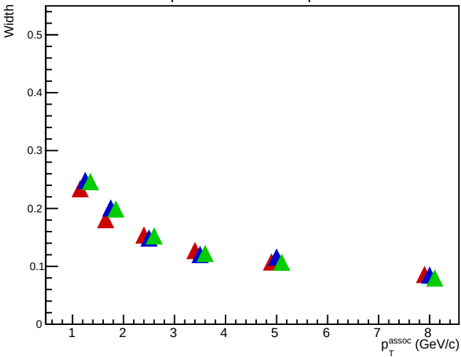
Widths vs p_T^{\text{assoc}} , Near Side, p_T^{\text{Jet, reco}} \in [20 \ 40]
