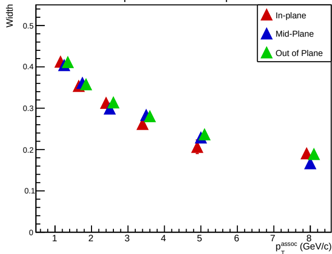
Widths vs p_T^{\text{assoc}} , Away Side, p_T^{\text{Jet, reco}} \in [15 \ 20]
