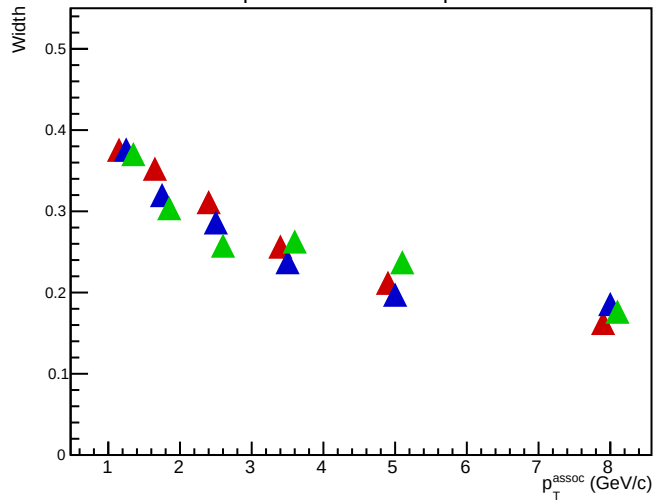
Widths vs p_T^{\text{assoc}} , Away Side, p_T^{\text{Jet, reco}} \in [20 \ 40]
