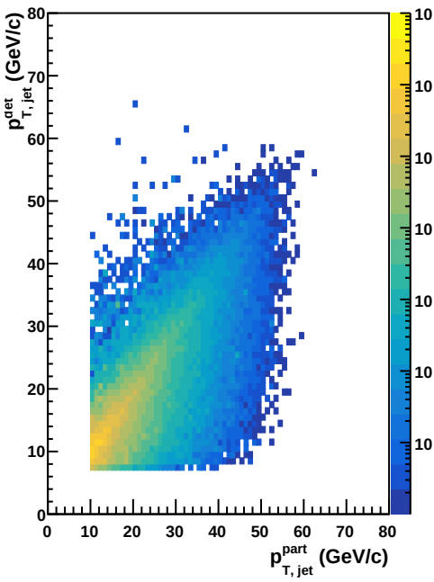
p_{T,jet}^{part} vs p_{T,jet}^{det} , in-plane
