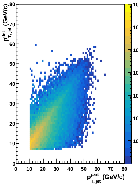
p_{T,jet}^{part} vs p_{T,jet}^{det} , mid-plane
