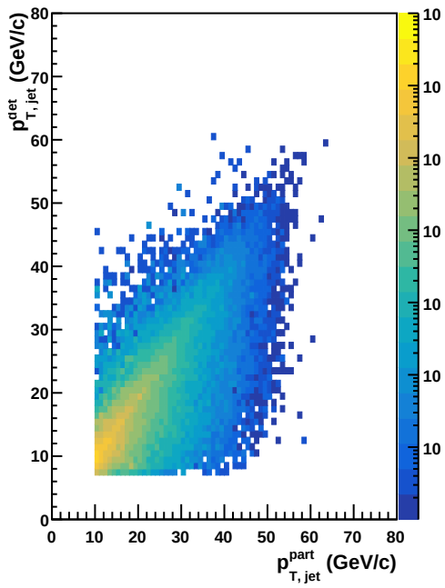
p_{T,jet}^{part} vs p_{T,jet}^{det} , out-plane
