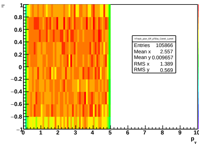
Track efficiency: cent = 4, lumi = 4, pion
