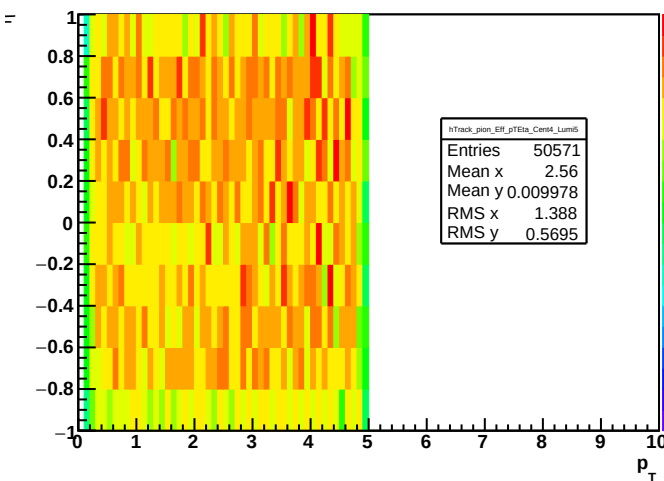
Track efficiency: cent = 4, lumi = 5, pion
