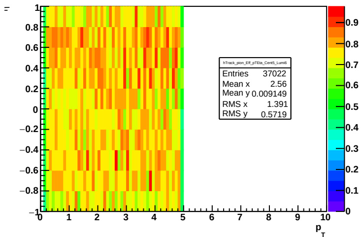
Track efficiency: cent = 5, lumi = 6, pion
