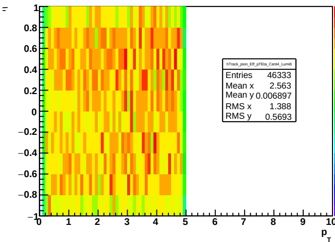
Track efficiency: cent = 4, lumi = 6, pion
