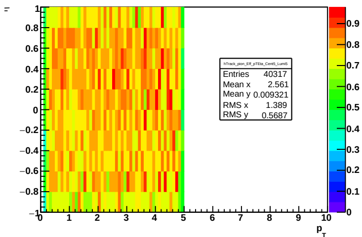
Track efficiency: cent = 5, lumi = 5, pion
