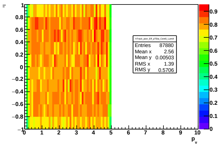
Track efficiency: cent = 5, lumi = 4, pion
