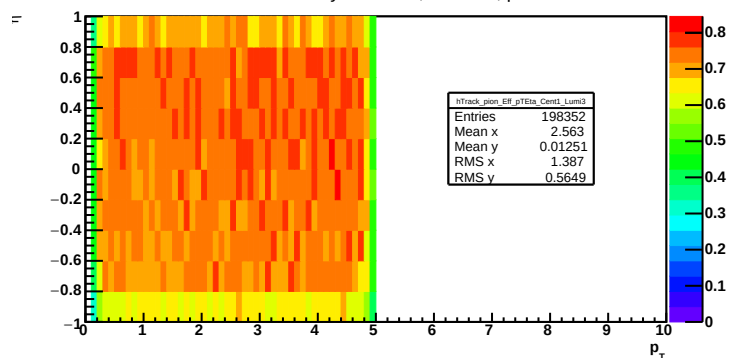
Track efficiency: cent = 1, lumi = 3, pion
