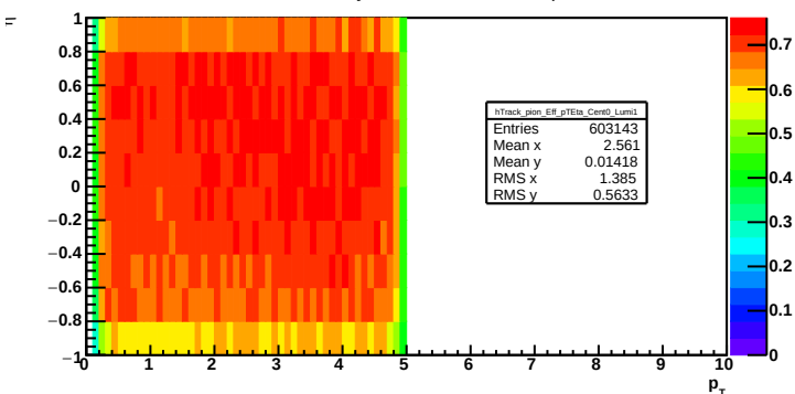
Track efficiency: cent = 0, lumi = 1, pion
