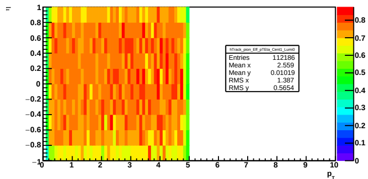
Track efficiency: cent = 1, lumi = 0, pion
