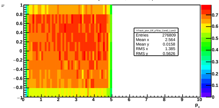
Track efficiency: cent = 0, lumi = 3, pion
