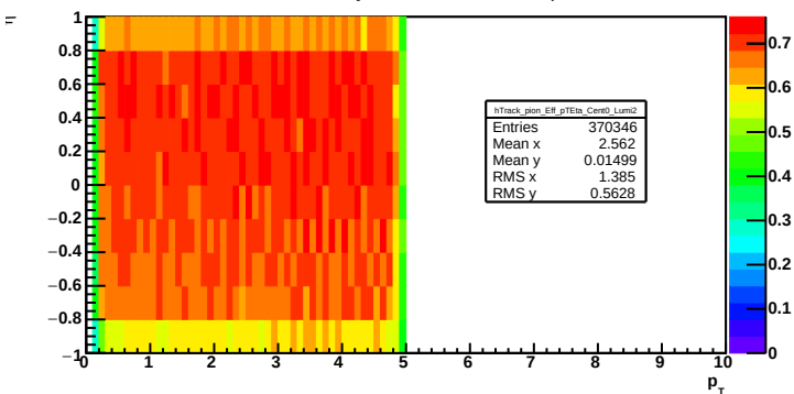
Track efficiency: cent = 0, lumi = 2, pion
