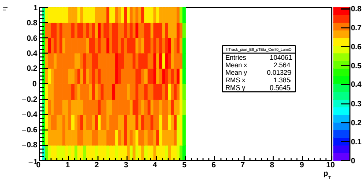
Track efficiency: cent = 0, lumi = 0, pion
