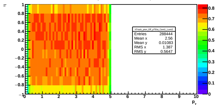
Track efficiency: cent = 1, lumi = 2, pion
