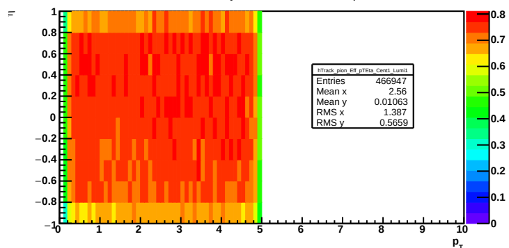
Track efficiency: cent = 1, lumi = 1, pion
