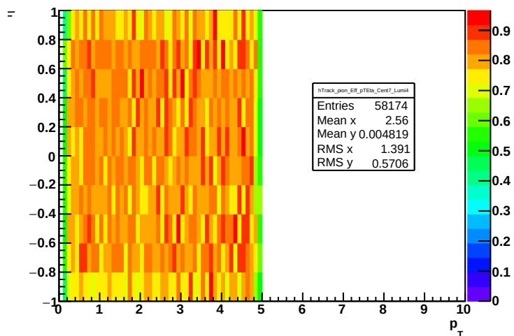
Track efficiency: cent = 7, lumi = 4, pion
