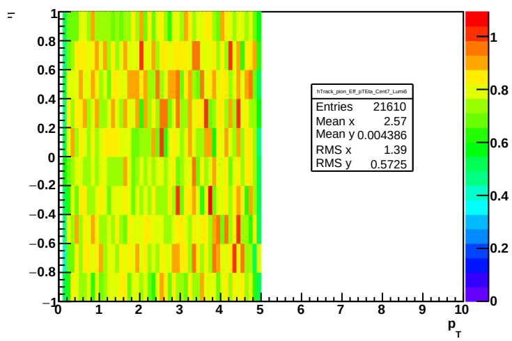
Track efficiency: cent = 7, lumi = 6, pion
