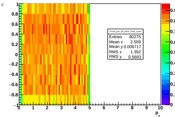
Track efficiency: cent = 6, lumi = 4, pion
