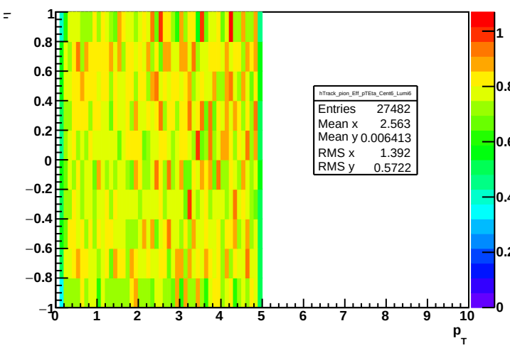
Track efficiency: cent = 6, lumi = 6, pion
