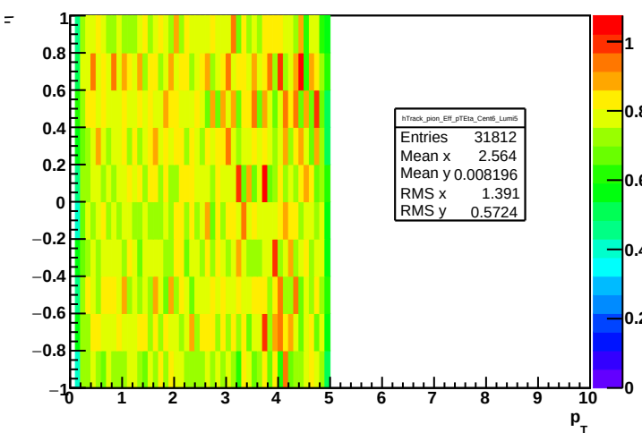
Track efficiency: cent = 6, lumi = 5, pion
