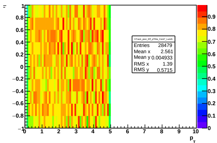
Track efficiency: cent = 7, lumi = 5, pion
