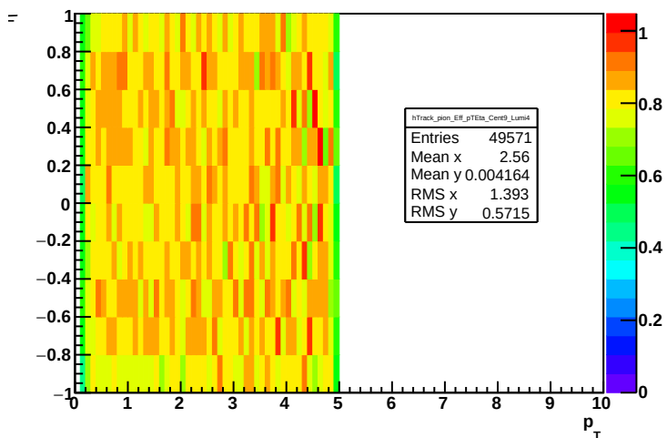
Track efficiency: cent = 9, lumi = 4, pion
