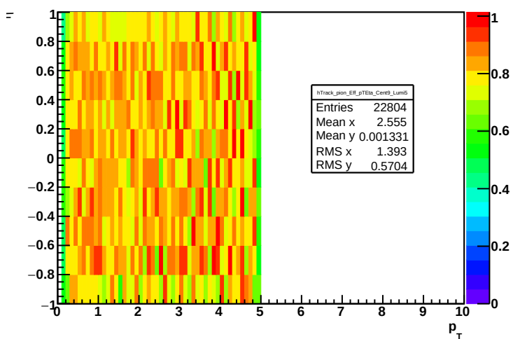
Track efficiency: cent = 9, lumi = 5, pion
