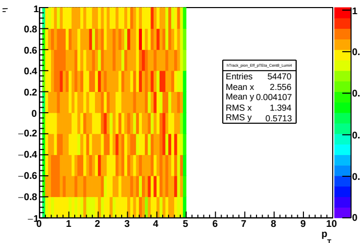
Track efficiency: cent = 8, lumi = 4, pion
