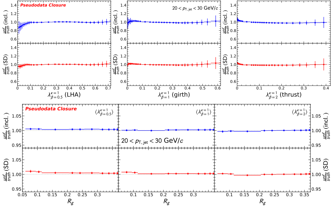
Figure 4.4: Closures for \lambda_{\beta \in \{0.5, 1, 2\}}^{\kappa=1} distributions (top) and R_g profile (bottom) shown for jets with 20 \leq p_{T,\text{jet}} < 30 \text{ GeV}/c .
