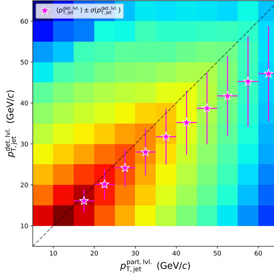
Figure 4.2: Two-dimensional histogram showing detector response for p_{T,\text{jet}} , showing probability of a p_{T,\text{jet}}^{\text{GEN}} particle level jet being reconstructed as p_{T,\text{jet}}^{\text{RECO}} . Purple stars shows expected p_{T,\text{jet}}^{\text{RECO}} given a particular bin of the p_{T,\text{jet}}^{\text{GEN}} .
