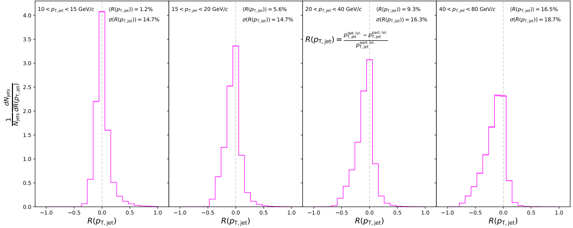
Figure 4.3: p_{T,\text{jet}} -resolution in different p_{T,\text{jet}} bins.
