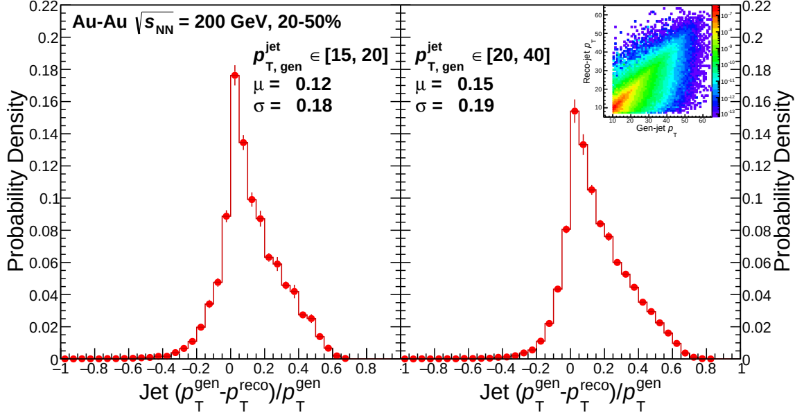
Figure 4.4: p_{T,\text{jet}} resolution for 15 < p_{T,\text{jet}}^{\text{GEN}} < 20 GeV/c (left) and 20 < p_{T,\text{jet}}^{\text{GEN}} < 40 GeV/c (right) R = 0.4 full jets with the corresponding response matrix as an inset on the top right. Jets are measured from all angles relative to the event plane in the 20-50% most central events. This comparison is for matched GEN-level to RECO-level jets.
