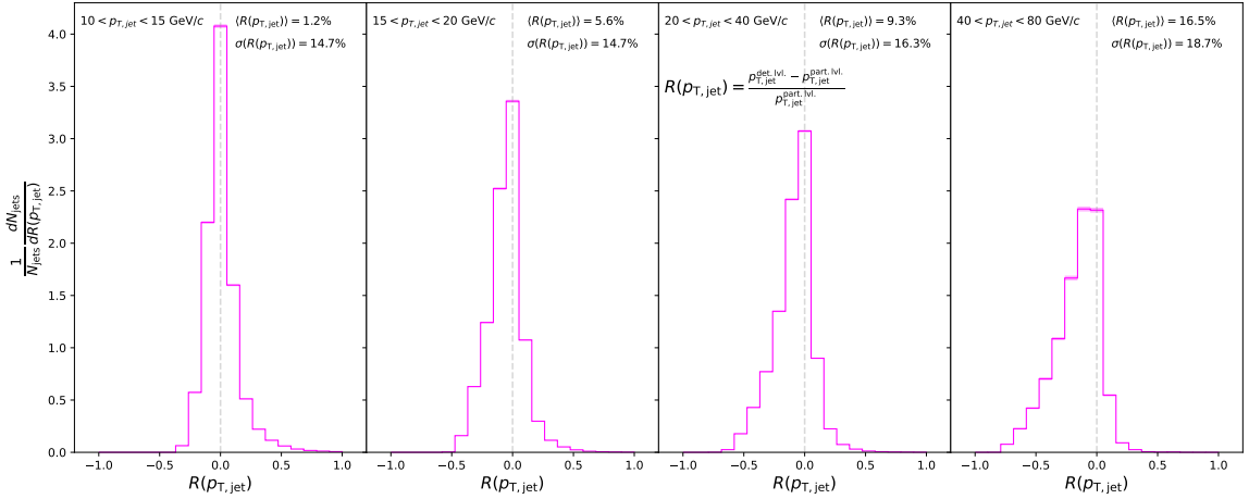
Figure 4.3: p_{T,jet} -resolution in different p_{T,jet} bins.
