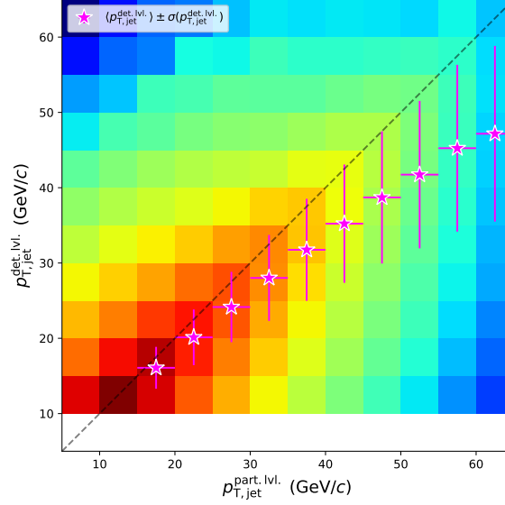
Figure 4.2: Two-dimensional histogram showing detector response for p_{T,jet} , showing probability of a p_{T,jet}^{GEN} particle level jet being reconstructed as p_{T,jet}^{RECO} . Purple stars shows expected p_{T,jet}^{RECO} given a particular bin of the p_{T,jet}^{GEN} .
