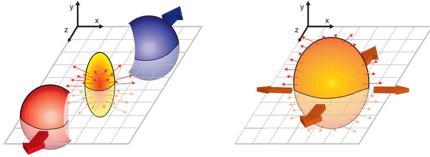
Figure 2.3: Typical heavy-ion collision
