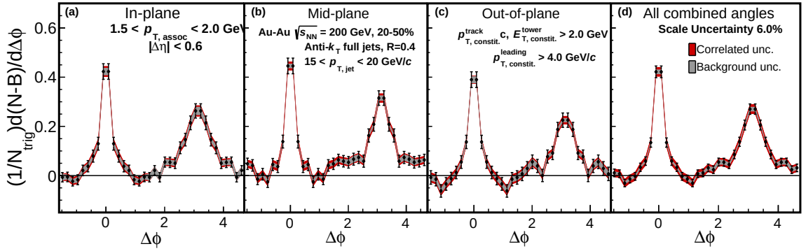
Figure 3.4: Example of a background subtracted correlation function for 15 < p_{T,\text{jet}} < 20 \text{ GeV}/c jets correlated with 1.5 < p_{T,\text{assoc}} < 2.0 \text{ GeV}/c charged hadrons from the 20-50% most central collisions. Correlated scaled uncertainty from the application of mixed events is displayed by the red band, while the uncertainty associated with the RPF background fit is displayed as the gray band.
