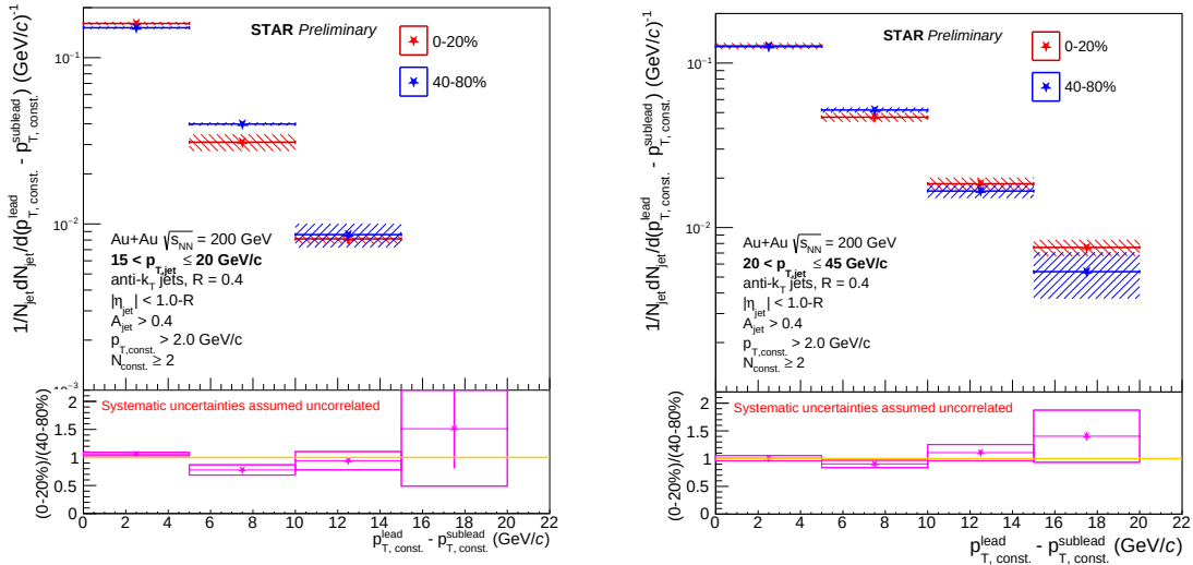
Figure 4.22: Normalized LeSub distributions for jets with 15 \leq p_{T,jet} < 20 GeV/c (left) and p_{T,jet} \geq 20 GeV/c (right) from central (0-20%, red stars) and peripheral (40-80%, blue stars) centrality ranges. Systematic uncertainties are shown as shaded boxes. Central over peripheral ratios (magenta stars) are in the lower panels with their systematic uncertainties represented as magenta boxes. Systematic uncertainties are assumed to be uncorrelated between the centrality ranges.
