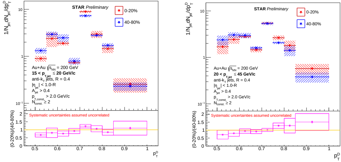
Figure 4.21: Normalized p_T^D = \sqrt{\lambda_0^2} distributions for jets with 15 \leq p_{T,jet} < 20 GeV/c (left) and p_{T,jet} \geq 20 GeV/c (right) from central (0-20%, red stars) and peripheral (40-80%, blue stars) centrality ranges. Systematic uncertainties are shown as shaded boxes. Central over peripheral ratios (magenta stars) are in the lower panels with their systematic uncertainties represented as magenta boxes. Systematic uncertainties are assumed to be uncorrelated between the centrality ranges.
