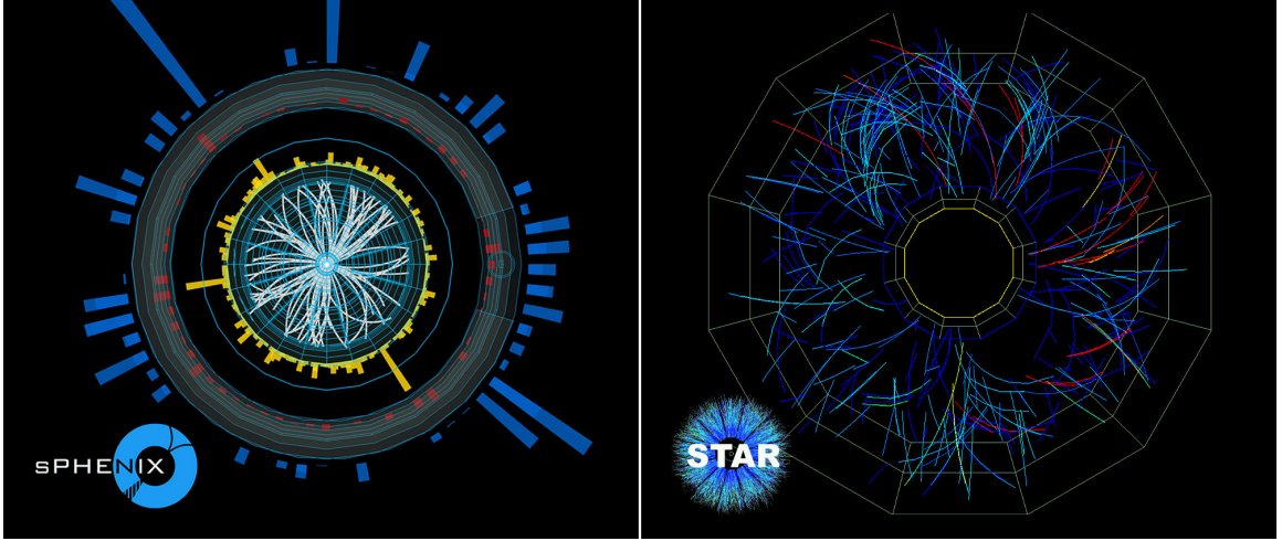
Figure 2.3: Some of the final O+O collisions at \sqrt{s_{\text{NN}}} = 200 GeV captured by the sPHENIX and STAR detectors at the RHIC. [14]
