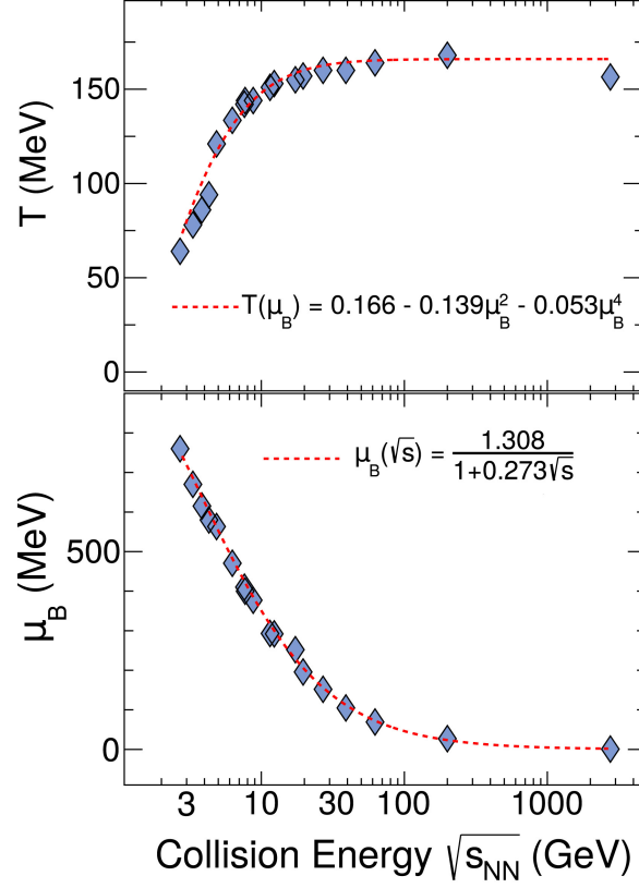
Figure 3.5: Chemical freeze-out parameters T and \mu_B obtained by thermal model fits to experimental data on particle yields as a function of collision energies. Red line represents parametrizations of T and \mu_B as a function of \sqrt{s_{NN}}
