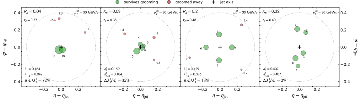
Figure 6.1: Ways of arranging constituents (each represented as a circle whose radius represent \frac{p_{T,const}}{p_{T,jet}} ) in the (\eta, \phi) space within a jet with p_{T,jet} = 30 \text{ GeV}/c such that R_g of the jet increases going from left to right. Green (Red) colored constituents survive (are removed by) the SoftDrop grooming ( z_{cut} = 0.2 , \beta = 0 ).
