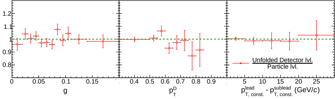
Figure 6.5: Closure test for g , p_T^D and LeSub showing the ratio of distributions calculated using jets from unfolded 0-20% centrality detector level and particle level events from Au+Au collisions at \sqrt{s_{NN}} = 200 GeV.
