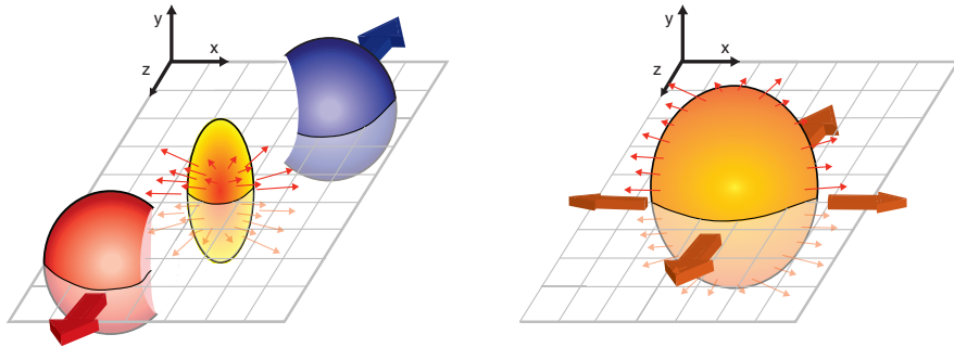
Figure 3.3: Schematic diagrams showing the initial overlap region (left) and the spatial anisotropy generated by this anisotropic overlap region. This anisotropy can be quantified using the Fourier coefficients of the momentum anisotropy.
