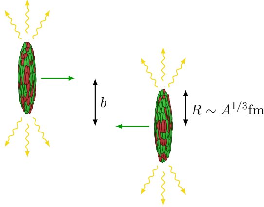
Figure 3.1: Typical heavy-ion collision
