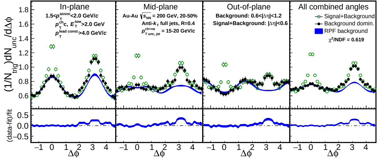
Figure 5.2: (Top) Signal+background region, background-dominated region, and RPF fit to the background for the event-plane dependent jet-hadron correlations of 15 < p_{T,jet}^{\text{jet}} < 20 GeV/ c jets correlated with 1.5 < p_{T,assoc} < 2.0 GeV/ c charged hadrons from the 20-50% most central events. (Bottom) Quality of the RPF fit to the background-dominated region expressed as (data - fit) / fit.
