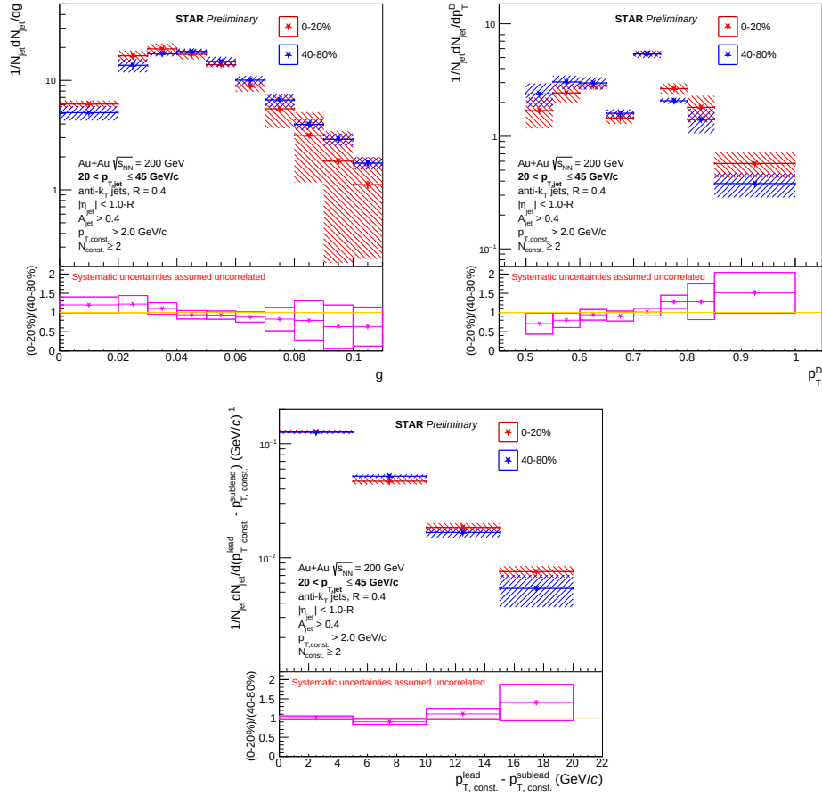
Figure 6.6: Normalized g , p_T^D and LeSub distributions for jets with p_{T,jet} \geq 20 GeV/c from central (0-20%, red stars) and peripheral (40-80%, blue stars) centrality ranges. Systematic uncertainties are shown as shaded boxes. Central over peripheral ratios (magenta stars) are in the lower panels with their systematic uncertainties represented as magenta boxes. Systematic uncertainties are assumed to be uncorrelated between the centrality ranges.
