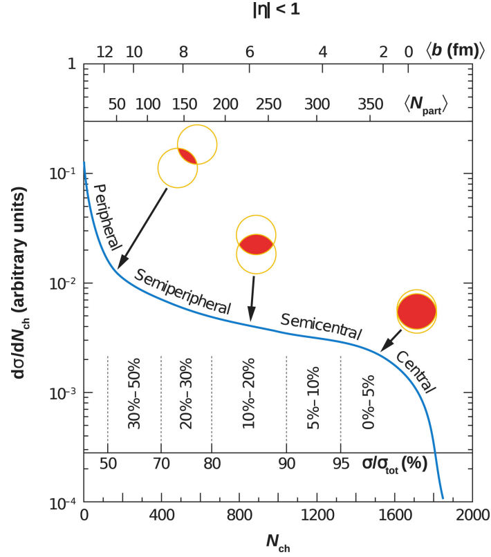
Figure 3.2: An illustration of the total inclusive charged particles multiplicity N_{\text{ch}} and number of participants ( N_{\text{part}} ) and impact parameter ( b ) in heavy-ion collisions
