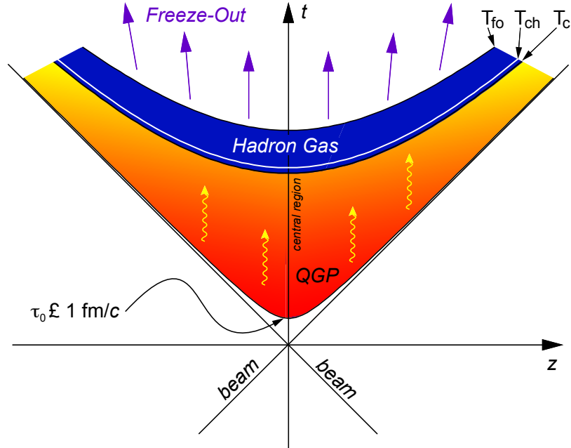
Figure 3.4: A light cone diagram showing the stages of a heavy ion collision. The abbreviation T_{fo} is for the thermal freeze-out temperature, T_{ch} is for the chemical freeze-out temperature, and T_c is for the critical temperature where the phase transition between a hadron gas and a QGP occurs. \tau_0 is the formation time of the QGP.
