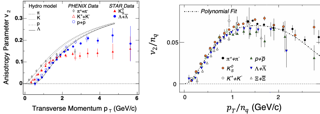
Figure 3.7: Left panel: Elliptic flow v_2 for several particle species in Au + Au collisions at \sqrt{s_{\text{NN}}} = 200 GeV from STAR and PHENIX experiments. Predictions from hydrodynamic models are shown as lines. Taken from [11]. Right panel: Number of constituent quarks ( n_q ) scaled v_2 as a function of p_T/n_q . Taken from [12].
