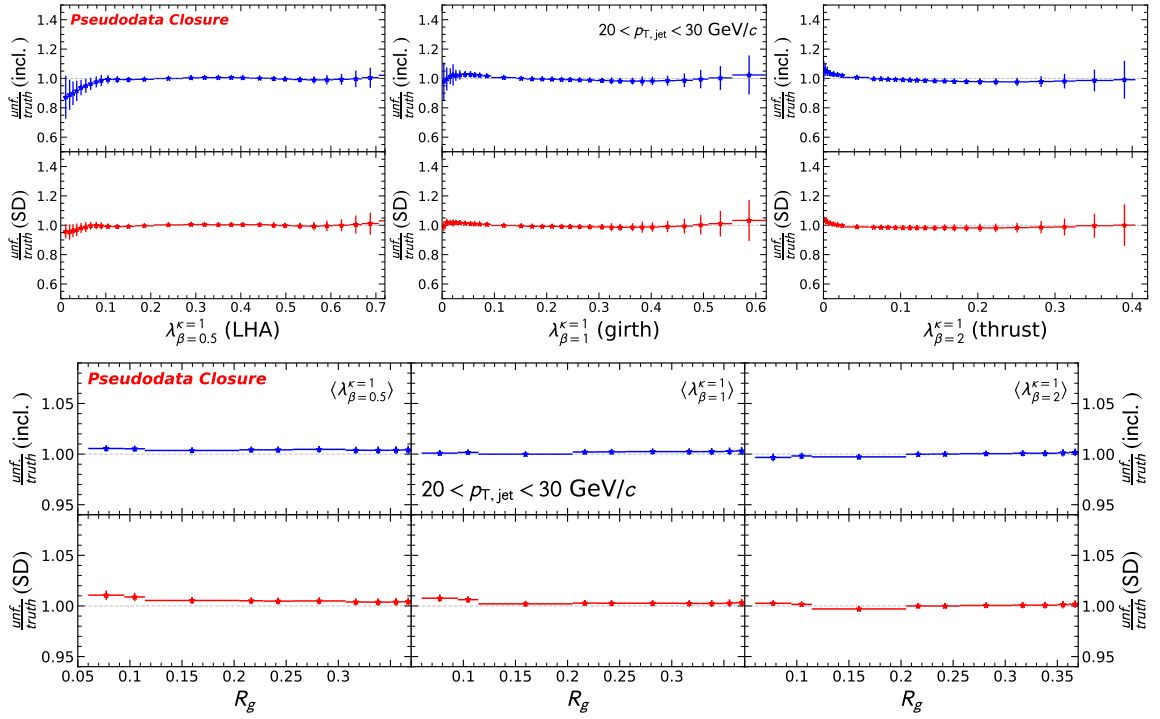
Figure 6.4: Closures for \lambda_{\beta=0.5,1,2}^{\kappa=1} distributions (top) and R_g profile (bottom) shown for jets with 20 \leq p_{T,jet} < 30 \text{ GeV}/c .
