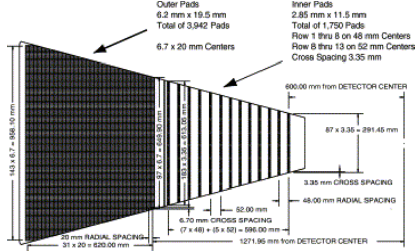
Figure 2.7: One of the twelve sectors of the TPC. Taken from [? ].
