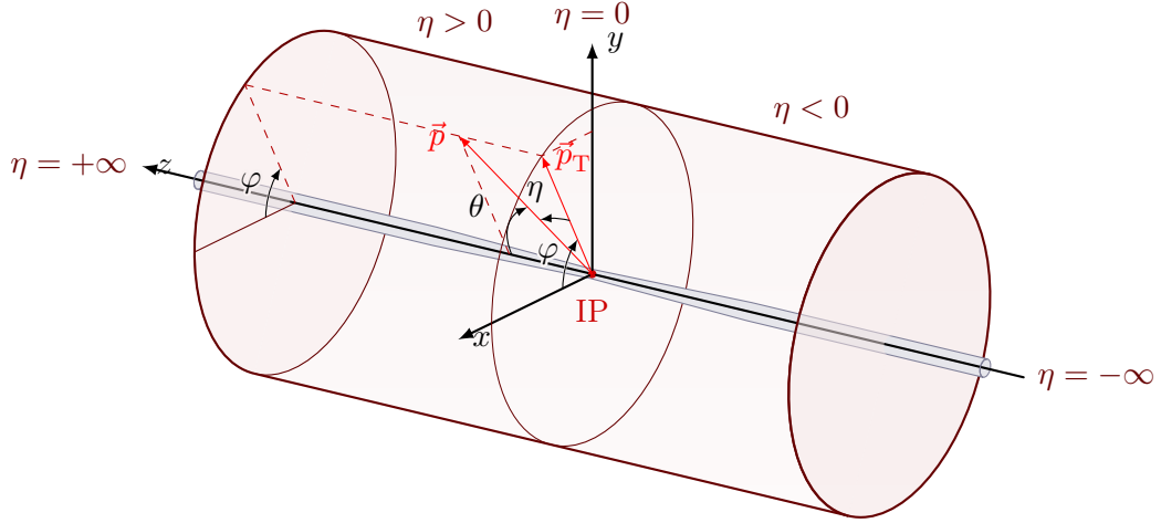
Figure A.2: The (p_T, \eta, \varphi) coordinate system, drawn for a cylindrical collider detector. The beam axis defines z and the interaction point (IP) sits at the origin. A particle of momentum \vec{p} is described by its transverse momentum \vec{p}_T , its azimuthal angle \varphi in the transverse plane, and its pseudo-rapidity \eta , fixed by the polar angle \theta with respect to the beam.
