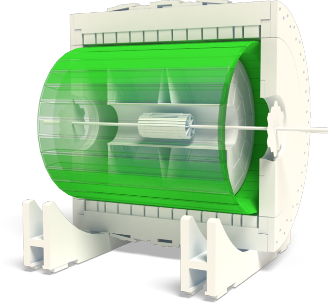
Figure 2.9: The Barrel Electromagnetic Calorimeter at STAR. Taken from [? ].
