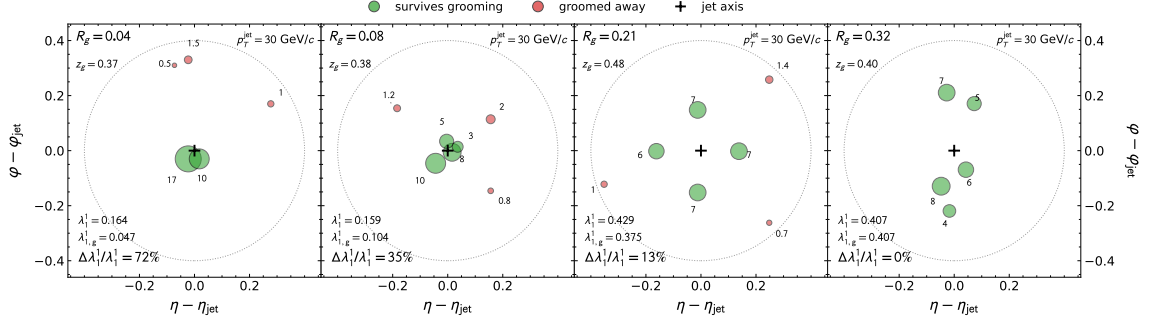
Figure 6.1: Ways of arranging constituents (each represented as a circle whose radius represent \frac{p_{T, \text{const}}}{p_{T, \text{jet}}} ) in the (\eta, \phi) space within a jet with p_{T, \text{jet}} = 30 \text{ GeV}/c such that R_g of the jet increases going from left to right. Green (Red) colored constituents survive (are removed by) the SoftDrop grooming ( z_{\text{cut}} = 0.2 , \beta = 0 ).
