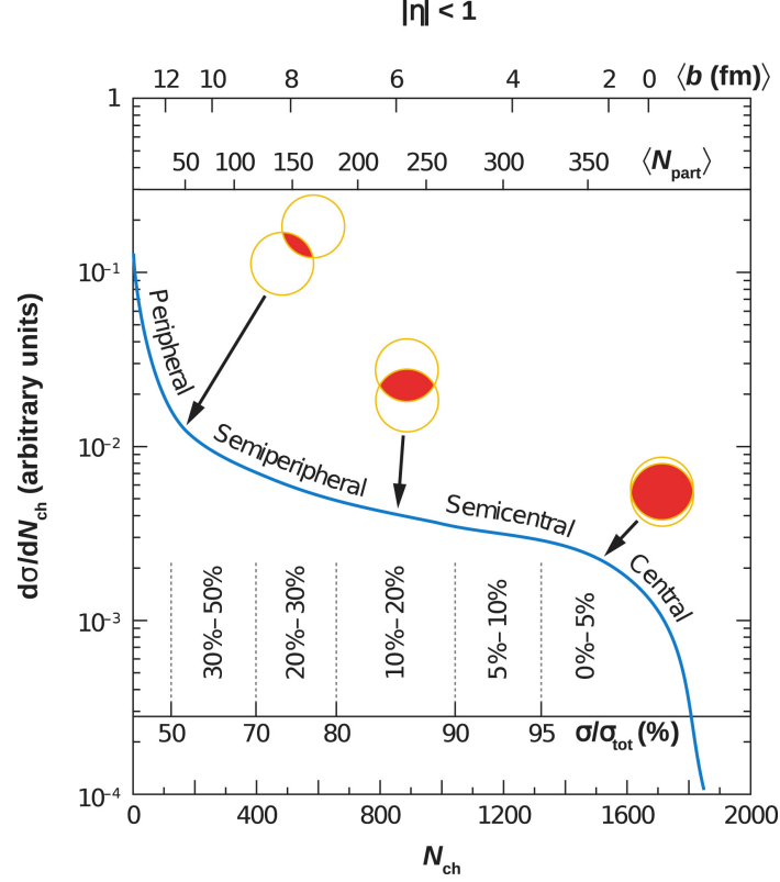
Figure 3.2: An illustration of the total inclusive charged particles multiplicity N_{\text{ch}} and number of participant ( N_{\text{part}} ) and impact parameter ( b ) in heavy-ion collisions
