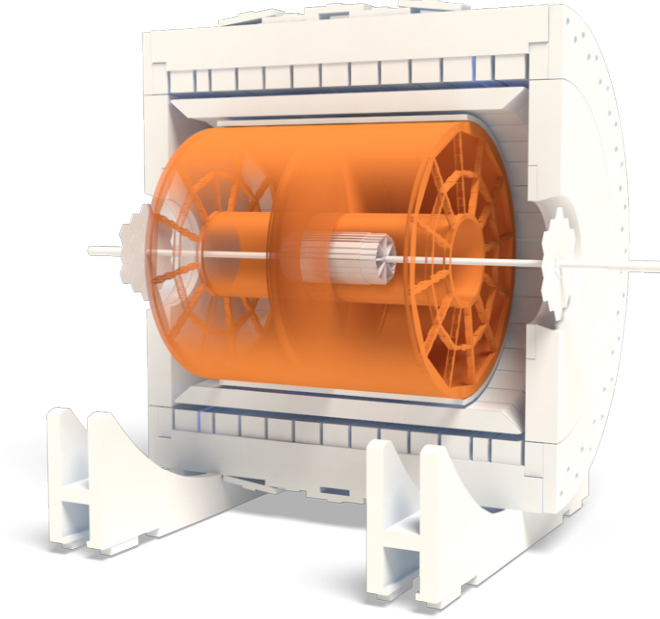
Figure 2.6: The Time Projection Chamber at STAR. Taken from [? ].
