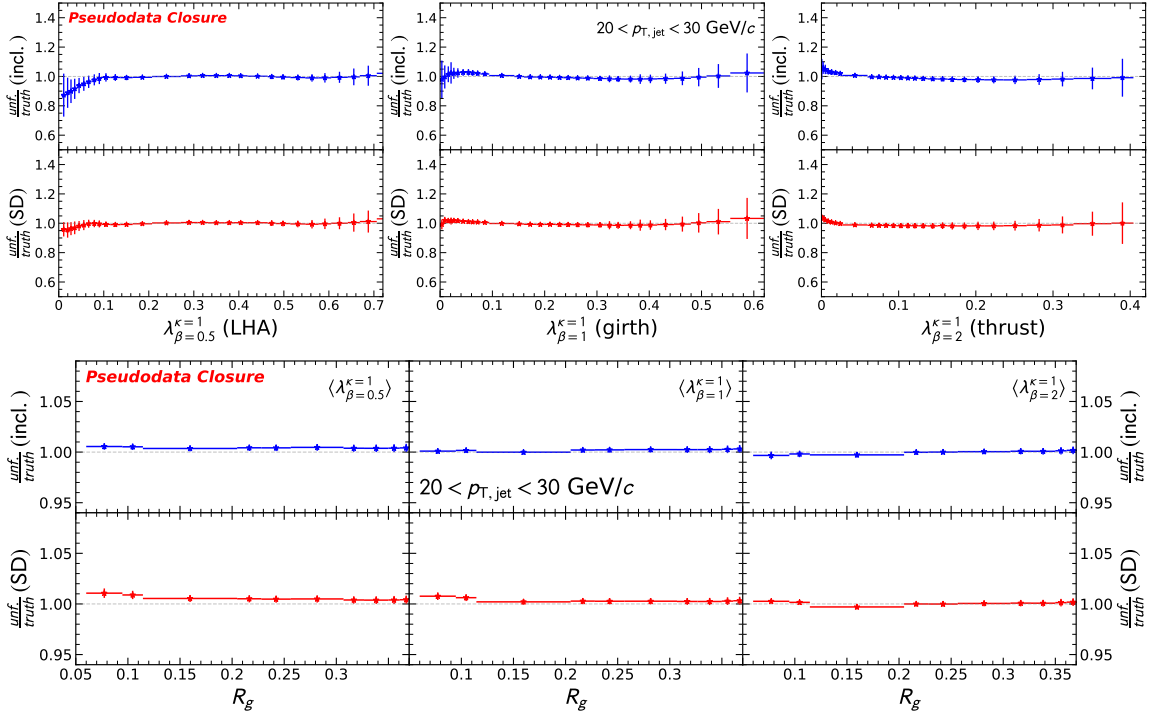
Figure 5.4: Closures for \lambda_{\beta \in \{0.5, 1, 2\}}^{\kappa=1} distributions (top) and R_g profile (bottom) shown for jets with 20 \leq p_{T,jet} < 30 \text{ GeV}/c .
