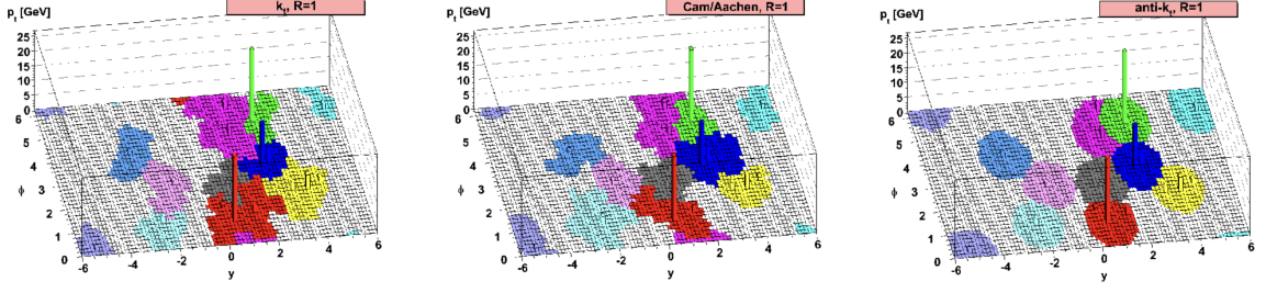
Figure 3.1: Jets reconstructed using the k_T (left), Cambridge/Aachen (middle), and anti- k_T (right) algorithms.
