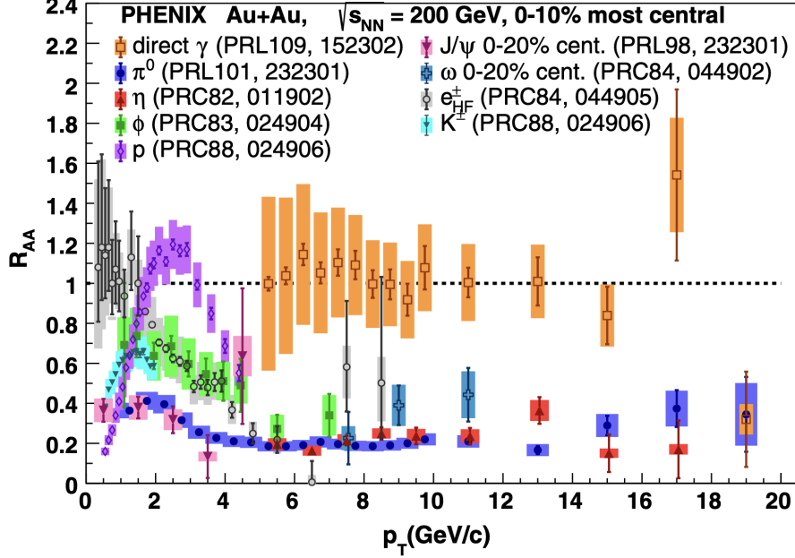
Figure 3.9: Nuclear modification factor R_{AA} as a function of p_T for identified particle species in Au + Au collisions at \sqrt{s_{NN}} = 200 GeV measured by the PHENIX experiment. Taken from [? ].
