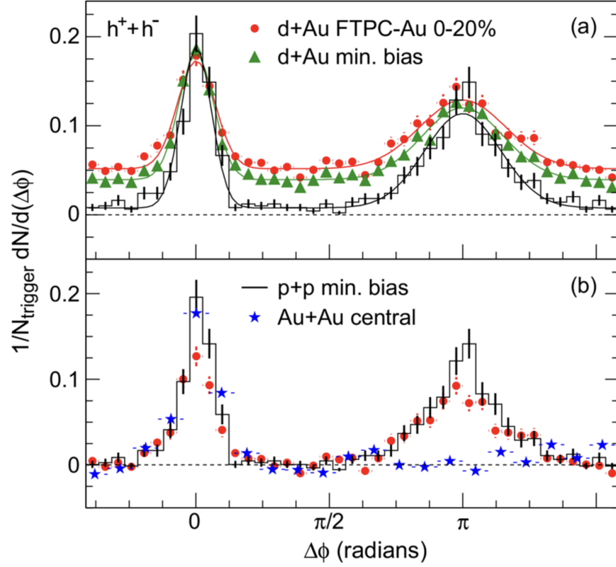
Figure 3.8: Measurement of the angular correlation between all charged hadrons and the leading hadron in the event for p + p (black lines), d + \text{Au} (red and green markers), and \text{Au} + \text{Au} events (blue markers), performed by the STAR experiment. The vanishing of the away-side yield around \Delta\phi \approx \pi in \text{Au} + \text{Au} events is evidence of particles getting quenched in the QGP medium. Taken from [? ].
