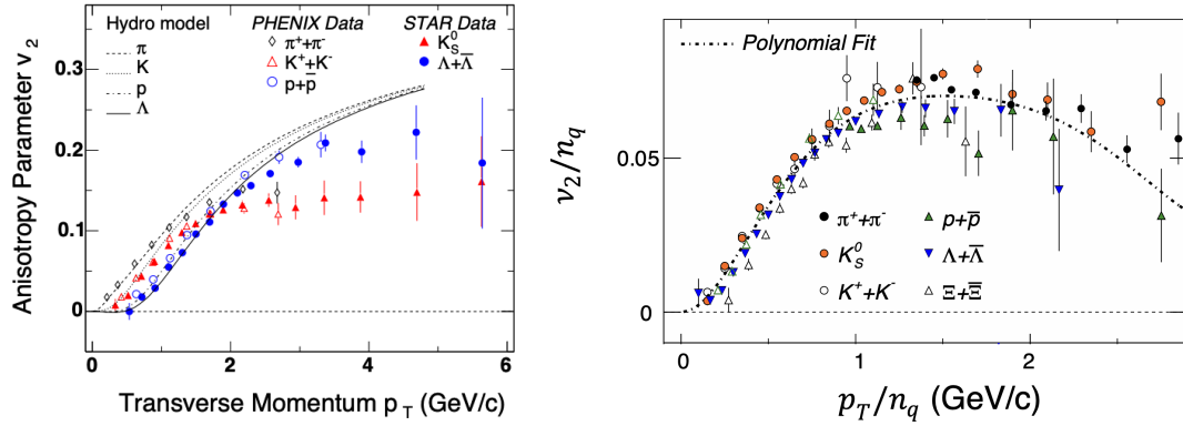
Figure 3.7: Left panel: Elliptic flow v_2 for several particle species in Au + Au collisions at \sqrt{s_{NN}} = 200 GeV from STAR and PHENIX experiments. Predictions from hydrodynamic models are shown as lines. Taken from [? ]. Right panel: Number of constituent quarks ( n_q ) scaled v_2 as a function of p_T/n_q . Taken from [? ].
