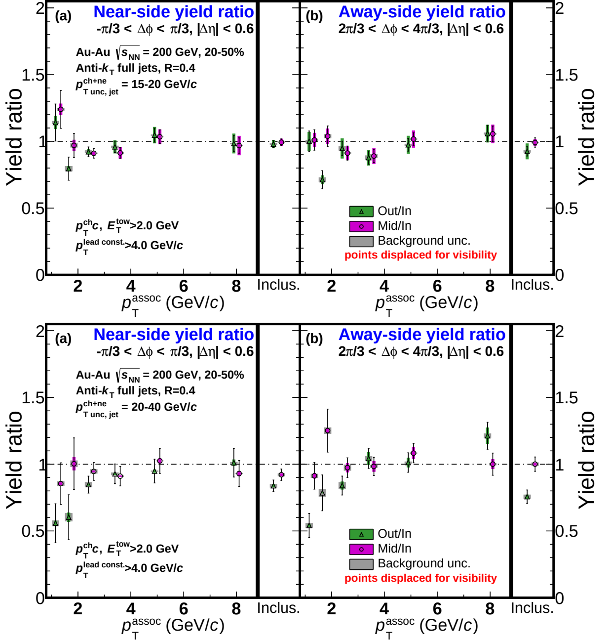
Figure 5.8: Near-side (left) and away-side (right) associated-yield ratios (of out-of-plane and mid-plane to in-plane) vs p_{T,assoc} for 15-20 (top) and 20-40 (bottom) GeV/c full jets in 20-50% centrality collisions. The grey bands describe the systematic uncertainties of the background fits which are non-trivially correlated point-to-point. The colored bands are scale uncertainties from the JES correction. Points are displaced for visibility.
