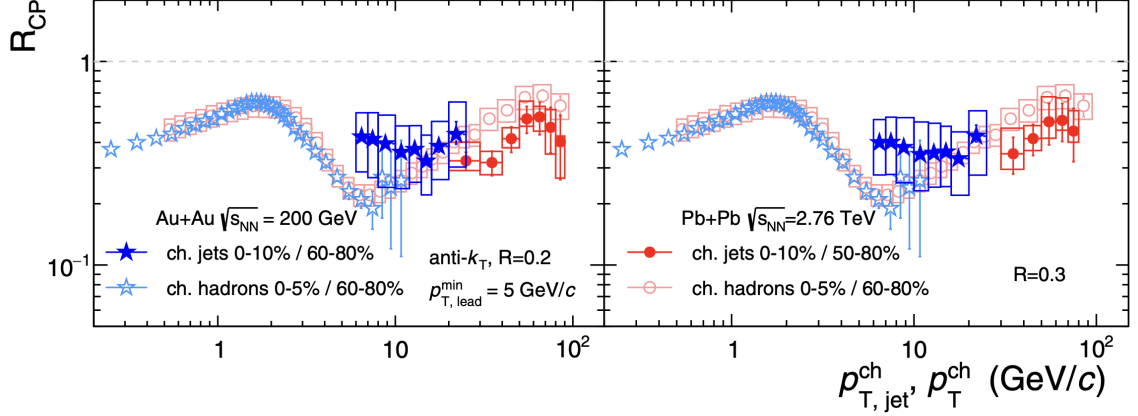
Figure 3.10: R_{CP} distributions for charged hadrons (open markers) and jets (solid markers) from RHIC (blue star markers) and LHC (red circle markers) experiments. Taken from [?] and references within [? ? ?].
