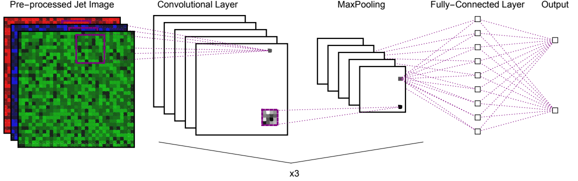
Figure 4.2: An illustration of the deep convolutional neural network architecture. The first layer is the input jet image, followed by three convolutional layers, a dense layer and an output layer. [8]
