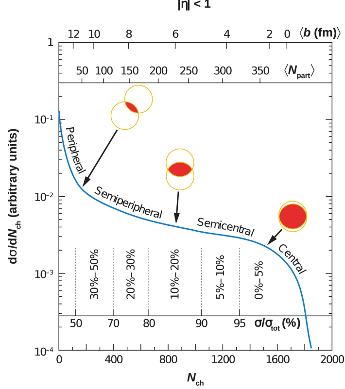
Figure 3.5: An illustration of the total inclusive charged particles multiplicity N_{ch} and number of participant ( N_{part} ) and impact parameter ( b ) in heavy-ion collisions
