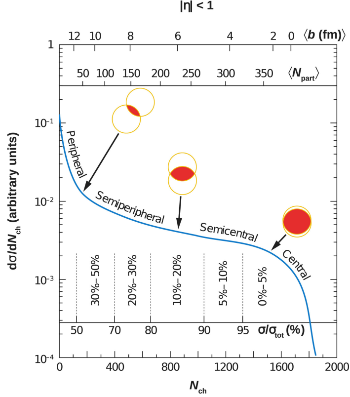
Figure 3.5: An illustration of the total inclusive charged particles multiplicity N_{ch} and number of participant ( N_{part} ) and impact parameter ( b ) in heavy-ion collisions. Taken from [10]
