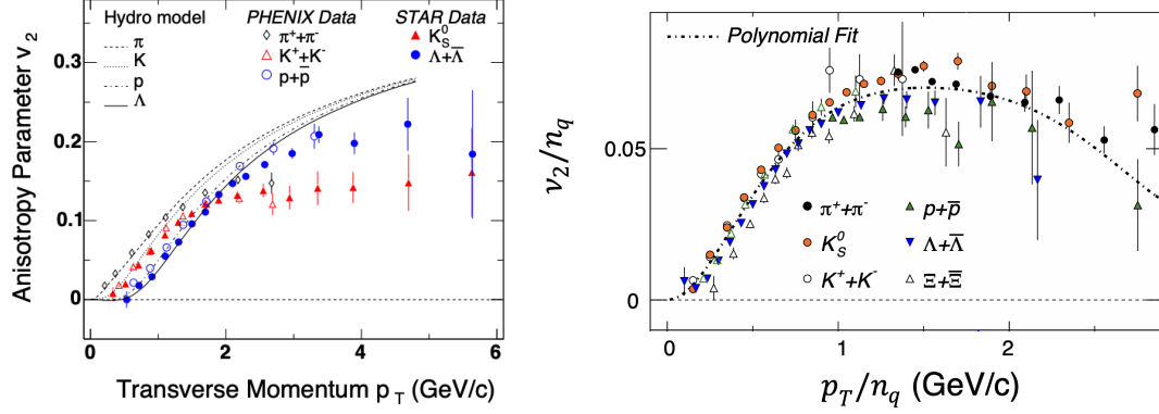
Figure 3.7: Left panel: Elliptic flow v_2 for several particle species in Au + Au collisions at \sqrt{s_{NN}} = 200 GeV from STAR and PHENIX experiments. Predictions from hydrodynamic models are shown as lines. Taken from [? ]. Right panel: Number of constituent quarks ( n_q ) scaled v_2 as a function of p_T/n_q . Taken from [? ].
