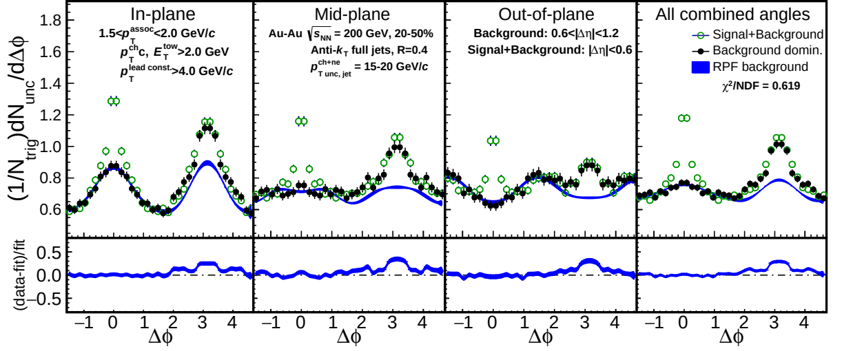
Figure 5.2: (Top) Signal+background region, background-dominated region, and RPF fit to the background for the event-plane dependent jet-hadron correlations of 15 < p_{T,\text{jet}}^{\text{jet}} < 20 GeV/ c jets correlated with p_{T,\text{assoc}} range 1.5-2.0 charged hadrons from the 20-50% most central events. (Bottom) Quality of the RPF fit to the background-dominated region expressed as (\text{data} - \text{fit}) / \text{fit} .
