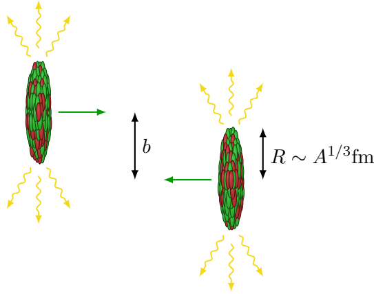
Figure 2.4: Typical heavy-ion collision
