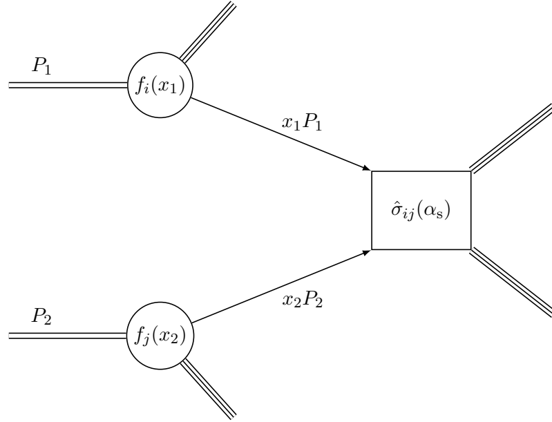
Figure 2.3: Collinear factorization of a hadronic hard scattering.
