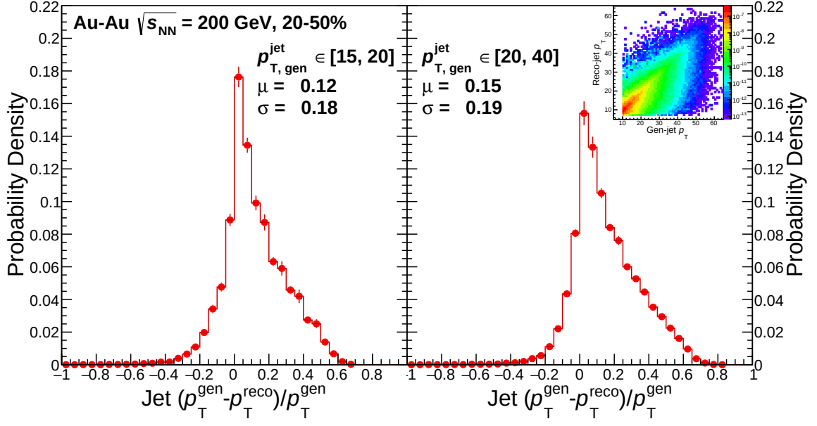
Figure 5.4 p_{T,jet} resolution for 15 < p_{T,jet}^{GEN} < 20 GeV/c (left) and 20 < p_{T,jet}^{GEN} < 40 GeV/c (right) R = 0.4 full jets with the corresponding response matrix as an inset on the top right. Jets are measured from all angles relative to the event plane in the 20-50% most central events. This comparison is for matched GEN-level to RECO-level jets.
