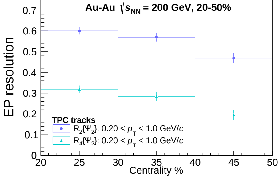
Figure 5.1 Event-plane resolution: Second-order (fourth-order) harmonic relative to the event plane, R_2(\Psi_2) ( R_4(\Psi_2) ), respectively. The approach follows the Modified Reaction Plane (MRP) method [1] utilizing the charged tracks of the TPC for event-plane reconstruction and resolution calculation for tracks ranging from 0.2-1.0 GeV/c.
