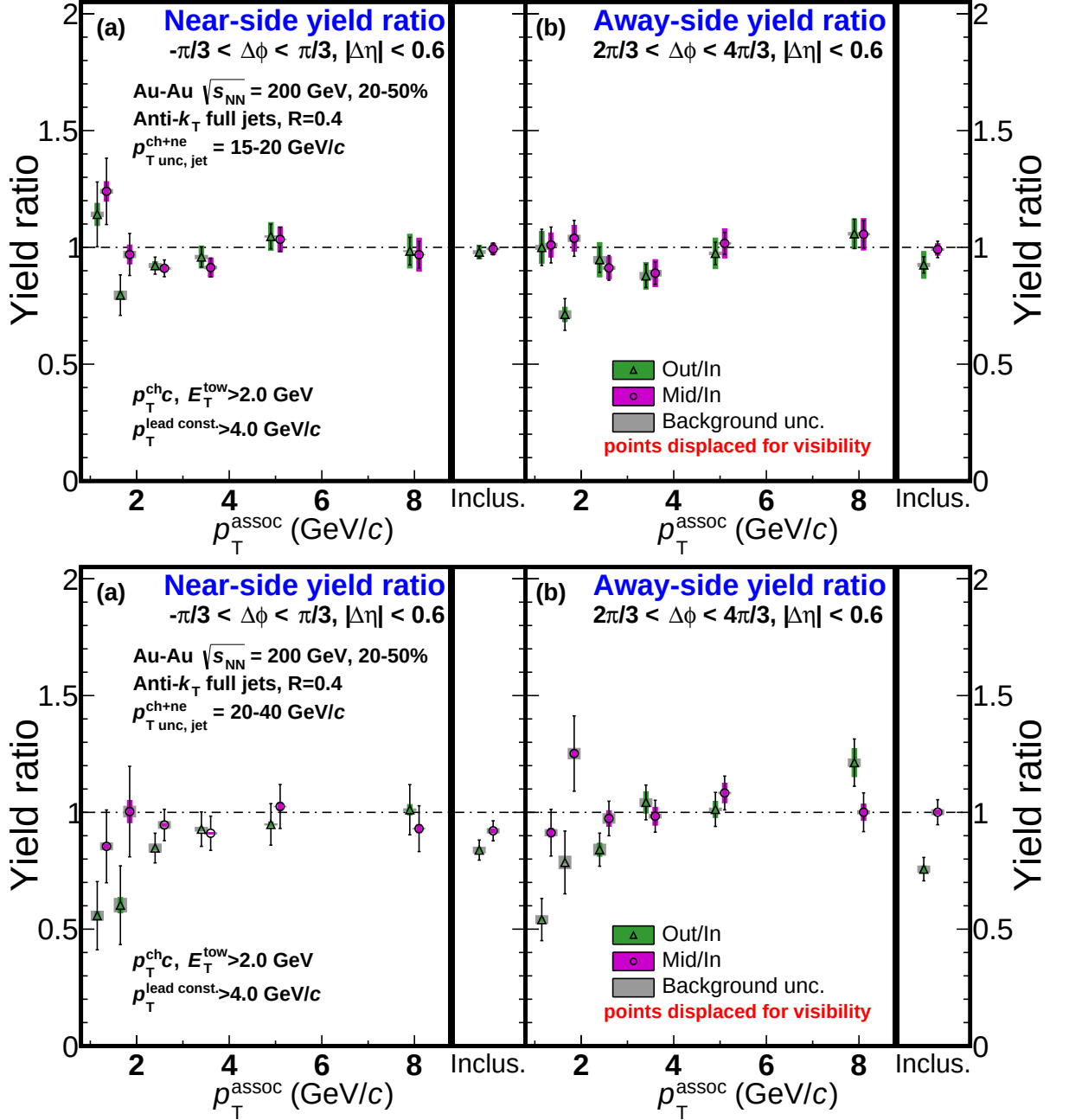
Figure 5.7: Near-side (left) and away-side (right) associated-yield ratios (of out-of-plane and mid-plane to in-plane) vs p_{T,assoc} for 15-20 (top) and 20-40 (bottom) GeV/ c full jets in 20-50% centrality collisions. The grey bands describe the systematic uncertainties of the background fits which are non-trivially correlated point-to-point. The colored bands are scale uncertainties from the JES correction. Points are displaced for visibility.
