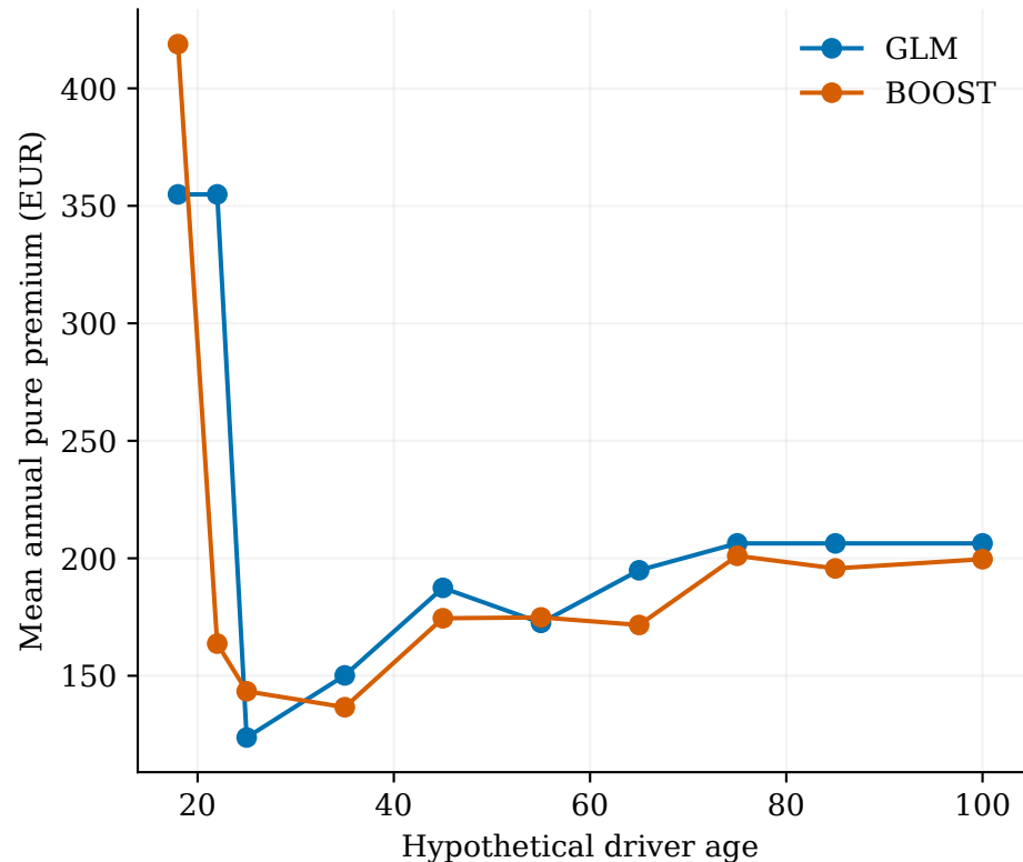
Age response: fixed validation risk sample
