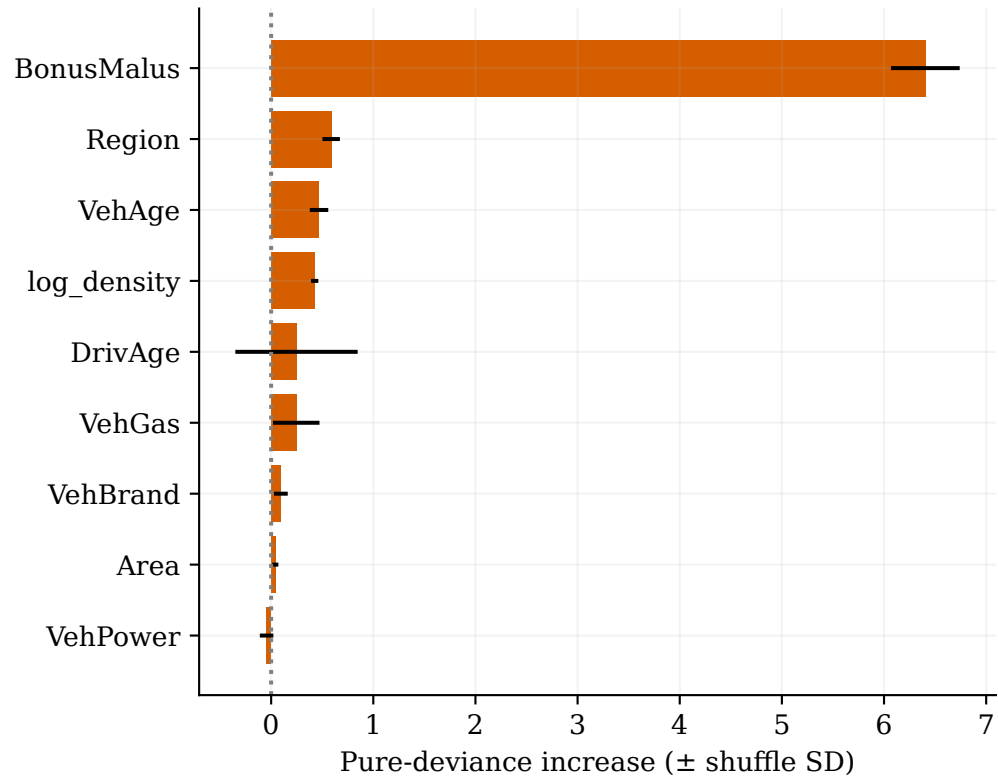
Boosting: validation permutation importance
