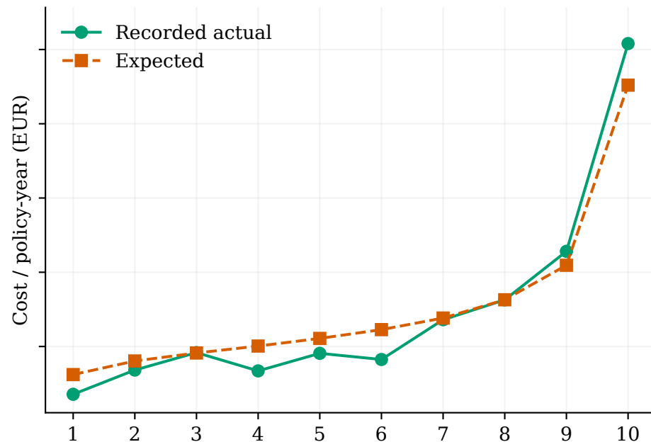
Final test: BOOST
