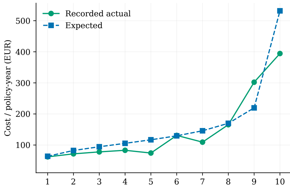
Final test: GLM
