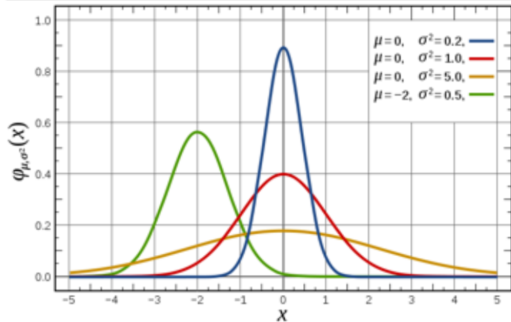
1-d Gaussian
