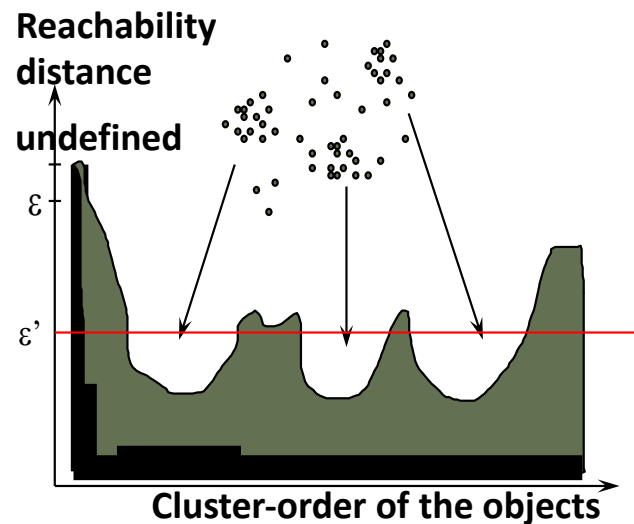
Figure 10.16: OPTICS terminology. Based on [ABKS99].
