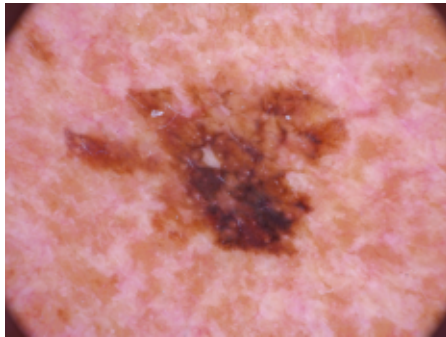
Original Image
