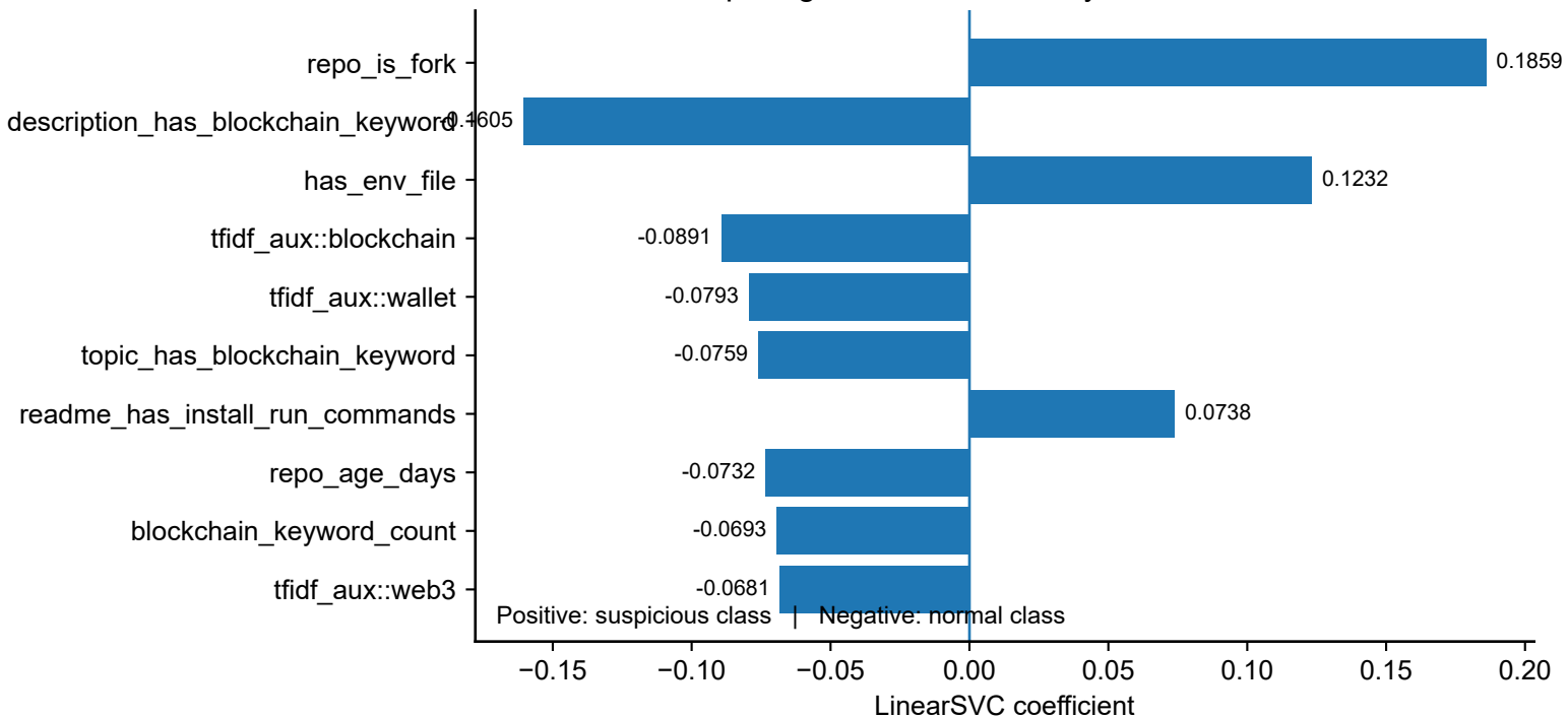
Top 10 global coefficients by absolute value
