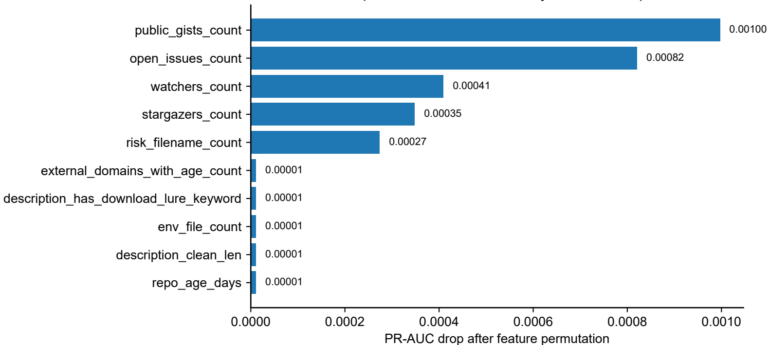
Top 10 structured features by PR-AUC drop
