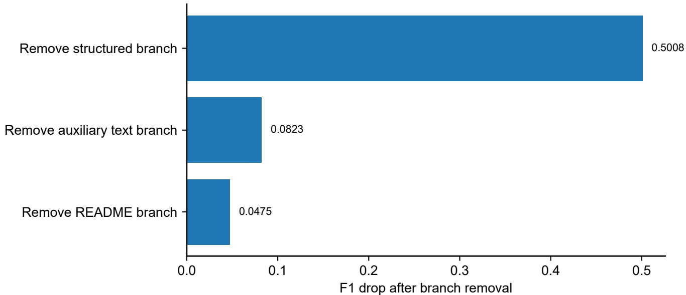
Branch ablation importance by F1 drop
