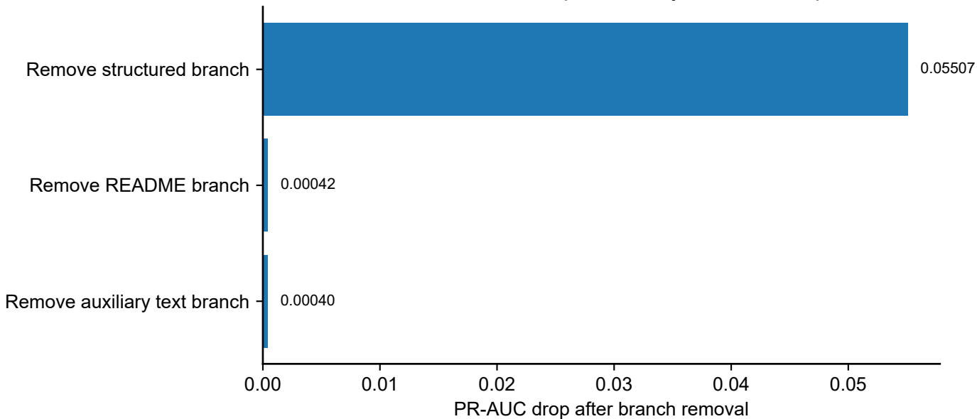
Branch ablation importance by PR-AUC drop
