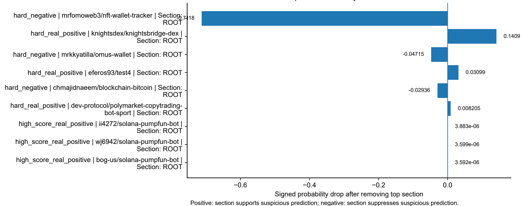
Top text sections by absolute effect
