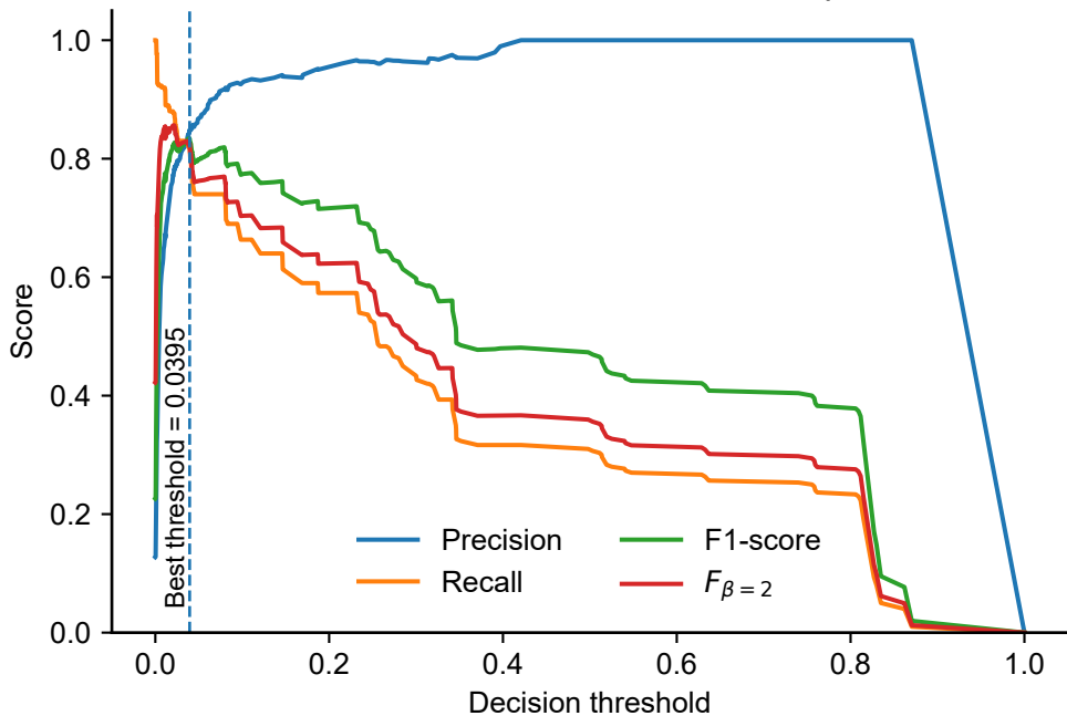
Threshold search curves based on OOF predictions
