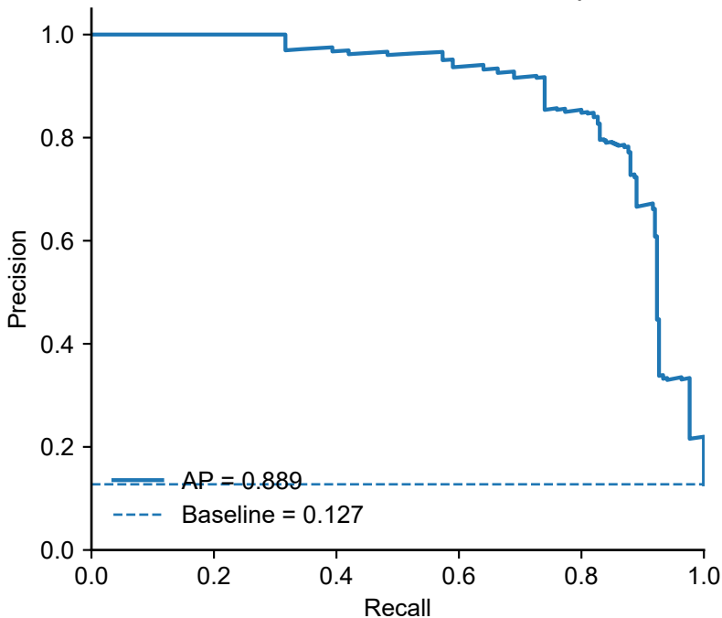
Precision-Recall curve based on OOF predictions
