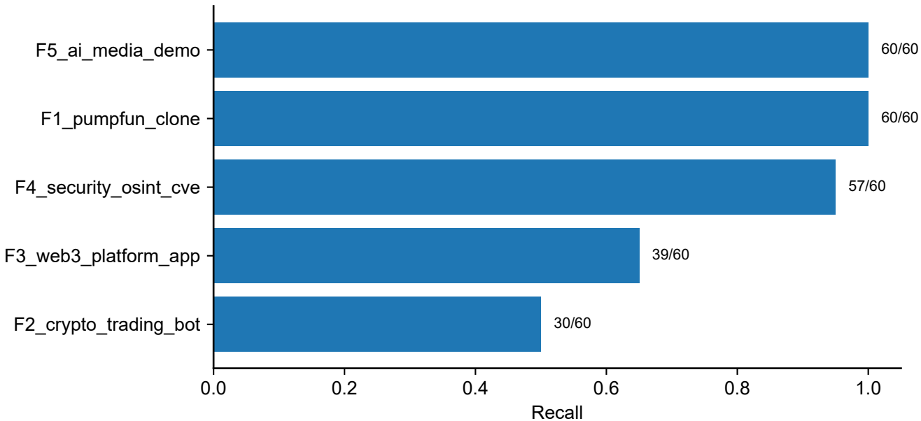
Positive recall by family (OOF validation)
