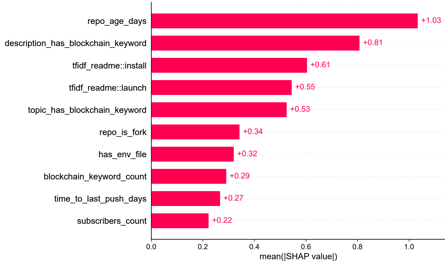
Global SHAP Importance (Top 10)
