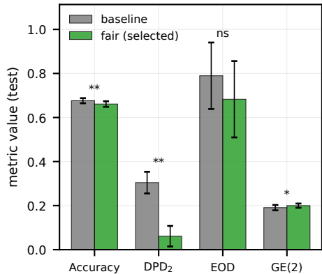
COMPAS
