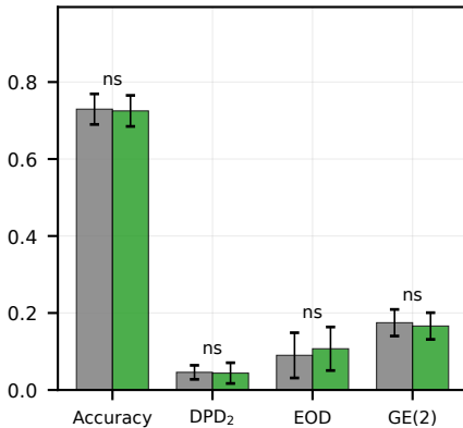
German Credit
