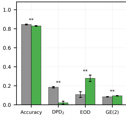
Adult
