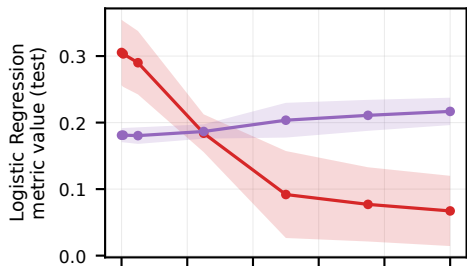
COMPAS
