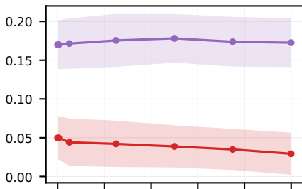
German Credit
