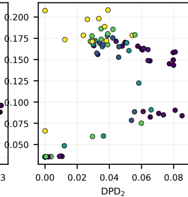
German Credit
