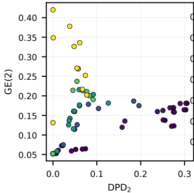
COMPAS
