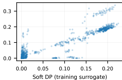
r = 0.923
