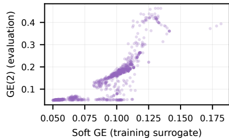
r = 0.832
