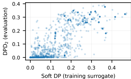
r = 0.832
