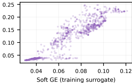
r = 0.919
