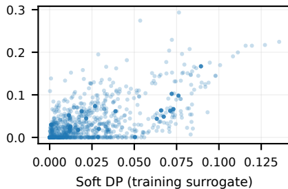
r = 0.919
