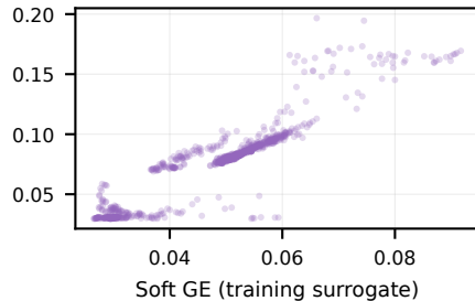
r = 0.923
