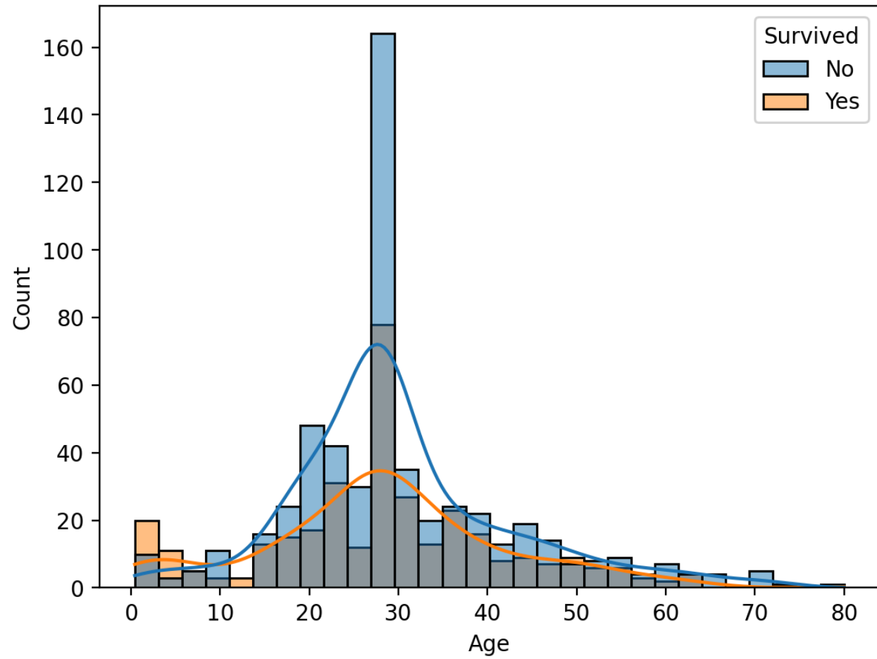
Age Distribution vs Survival
