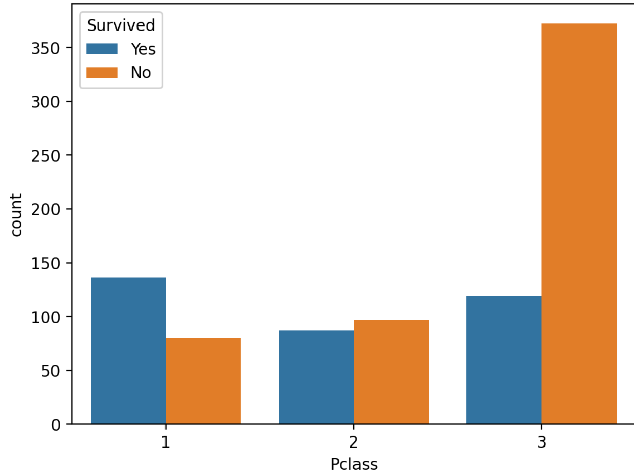
Survival by Passenger Class
