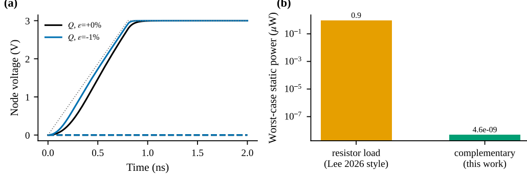
Figure S5: (a) Power-up restore transients for unstrained and -1\% strained latches. (b) Worst-case static power per stage: resistor load versus the complementary stage of this work.
