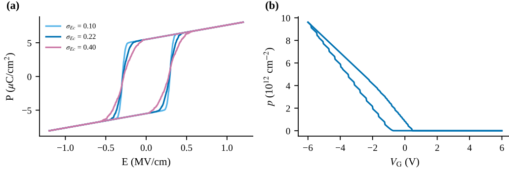
Figure S3: (a) Quasi-static P-E loops for three coercive-field spreads. (b) Channel hole density during the \pm 6 V double sweep of the baseline FeFET.
