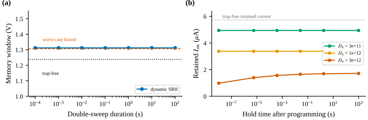
Figure S7: Finite-rate trap kinetics. (a) Memory window at D_{it} = 10^{12} \text{ cm}^{-2}\text{eV}^{-1} versus double-sweep duration: the kinetic result coincides with the quasi-static bound and stays within 6% of the trap-free window over six decades of sweep rate. (b) Retained on-current versus hold time after a 100 \mu\text{s} program pulse: emission of trap levels above the retained Fermi level recovers the read current toward its equilibrium value, keeping a working cell even at 3 \times 10^{12} \text{ cm}^{-2}\text{eV}^{-1} .
