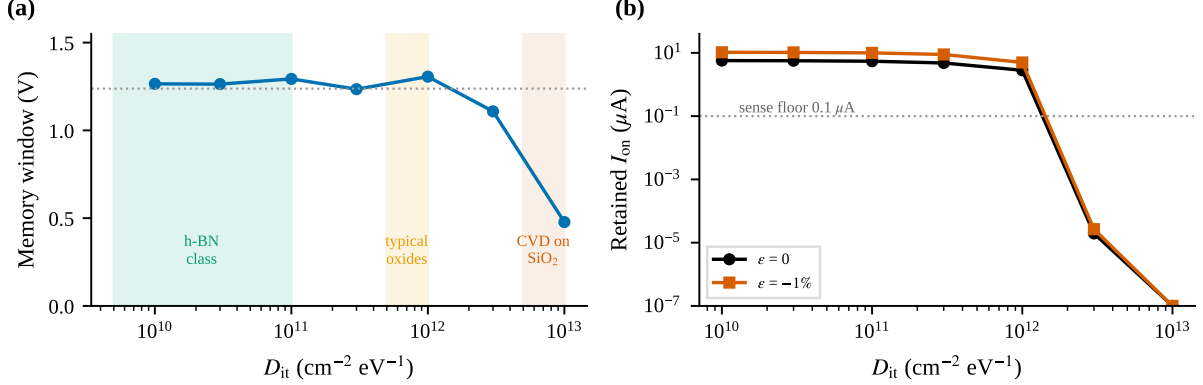
Figure S6: Worst-case interface-trap robustness. (a) Memory window versus trap density; shaded bands mark reported D_{it} ranges for h-BN-class interfaces, typical oxides, and CVD channels on SiO 2 . (b) Retained on-current at zero and -1\% strain; the logic-compatible regime persists up to 10^{12} cm -2 eV -1 .
