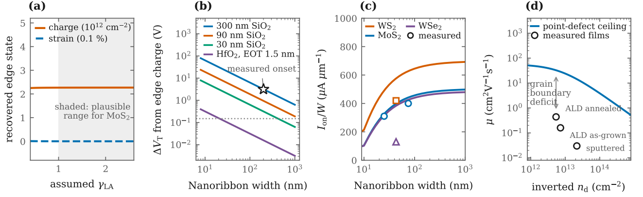
FIG. 3. Edge charge and its electrostatic signature. (a) Recovered edge carrier density and strain as the assumed acoustic Grüneisen parameter is scanned; the assignment is fixed by the unshifted overtone. (b) Threshold shift predicted by Eq. (1) for four gate stacks; the dotted line is ten per cent of the gate overdrive and the star marks the width at which a width-driven threshold shift was first reported. 8 (c) Predicted and measured on-current per unit width; measured points are the high- \kappa -gated devices of Ref. 5. (d) Defect densities inverted from the disorder-activated Raman ratio of published films, against their measured mobility and the point-defect ceiling.
