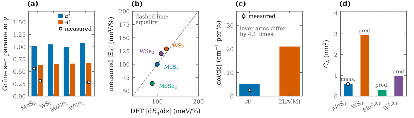
FIG. 2. First-principles deformation response. (a) Mode Grüneisen parameters from symmetric frozen-phonon calculations under biaxial strain, compared with direct measurements. (b) Computed strain derivative of the K -point gap against the measured A-exciton gauge factor for the same four materials; the dashed line is equality. (c) Strain sensitivity of the two Raman channels used here. (d) Disorder-activated Raman calibration constant: measured for MoS 2 , predicted here for the other three materials.
