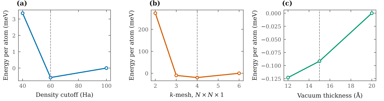
FIG. S1. Convergence for monolayer MoS 2 . (a) Energy per atom against the density-grid cutoff, referenced to 100 Ha. (b) Energy per atom against k -point sampling, referenced to a 6 \times 6 \times 1 mesh. (c) Energy per atom against vacuum thickness. Dashed lines mark the production settings.
