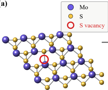
disordered monolayer MoS 2
