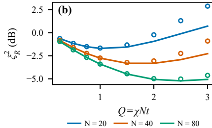
exact (circles) vs cumulant (lines)
