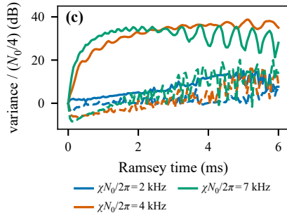
anti-squeezed (solid), squeezed (dashed)
