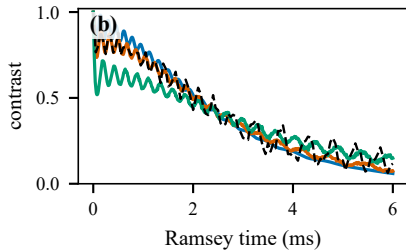
\chi N_0/2\pi = 7 kHz
